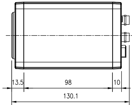
RIGHT
