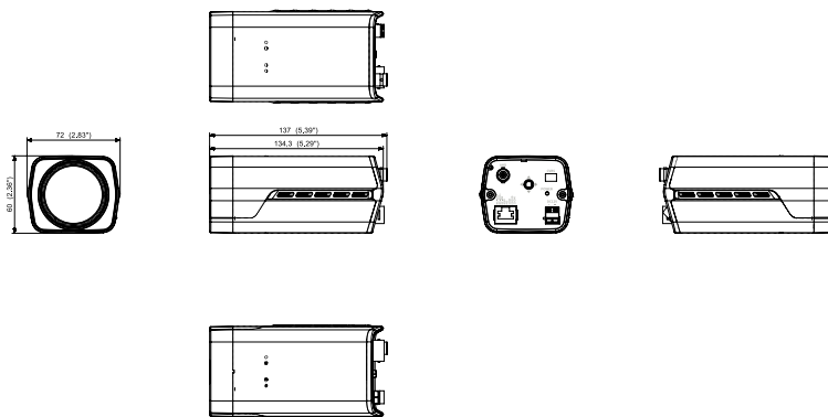
HCZ-6320 APPEARANCE
