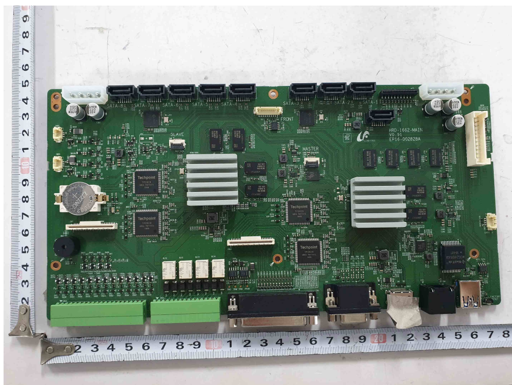
<Photo 6 > Main board Top
