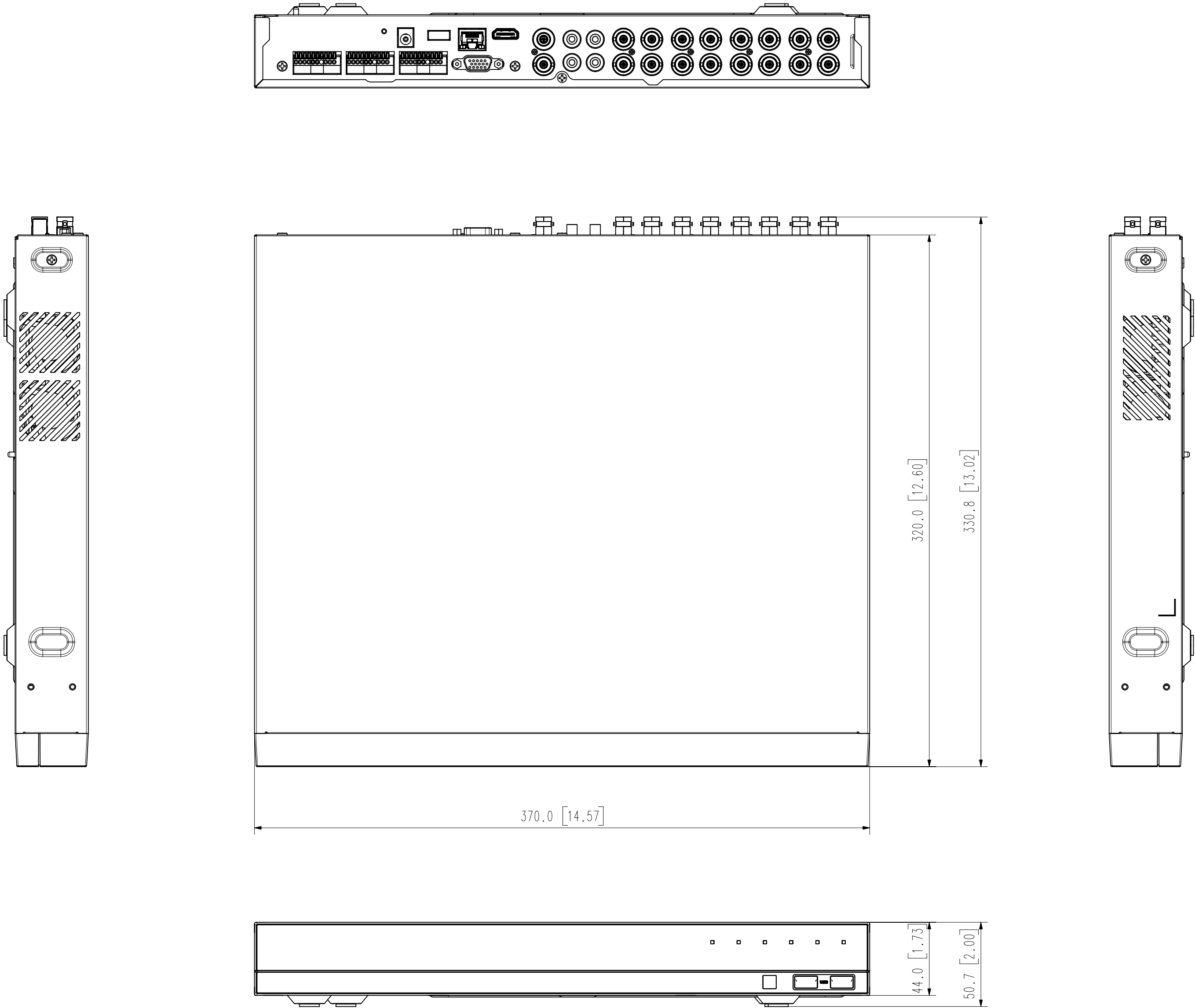
Appearance drawing HRX-1634 Unit : mm[inches]
