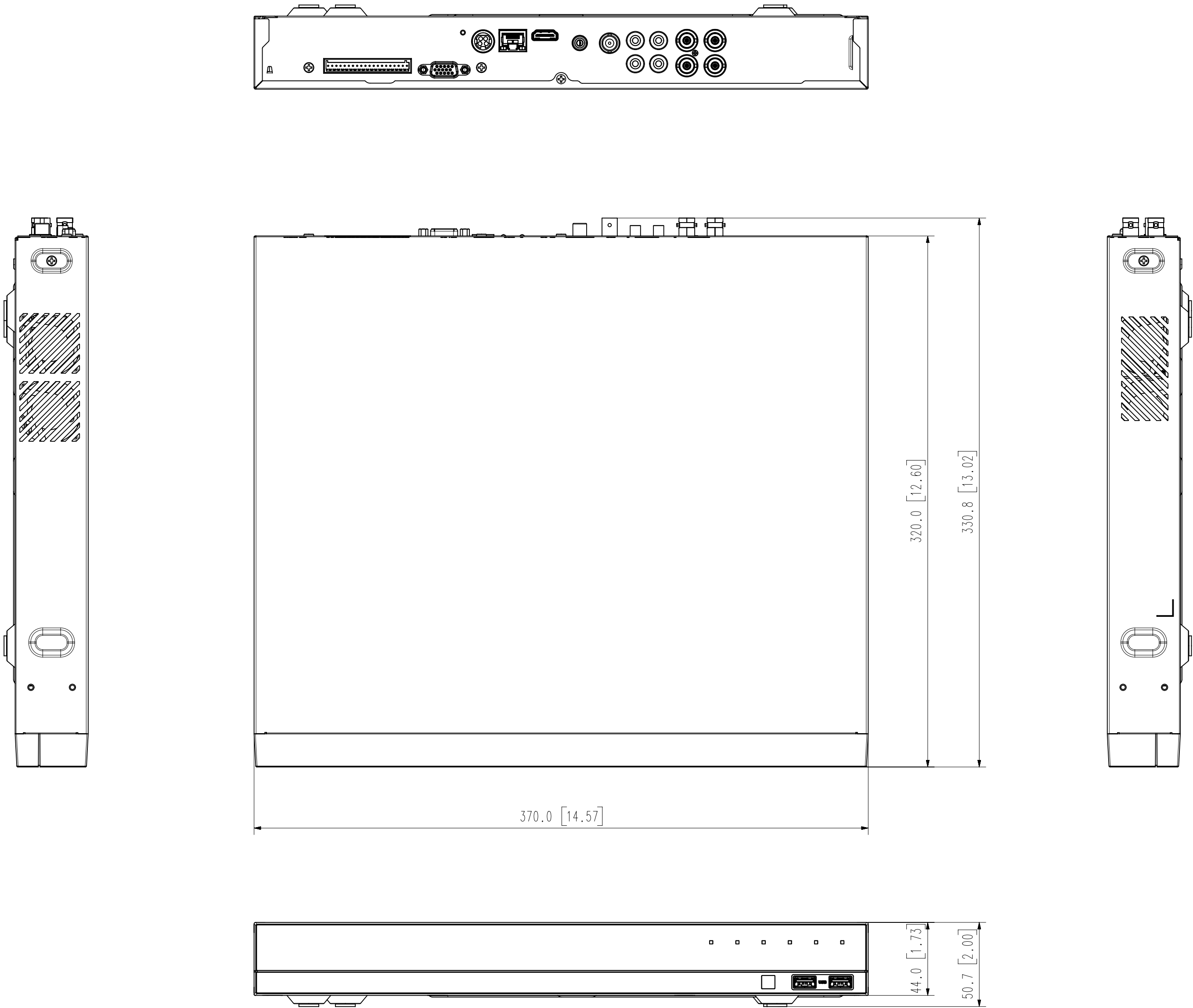
Appearance drawing HRX-435 Unit : mm[inches]
