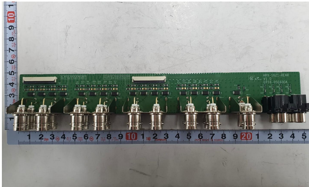
<Photo 17 > Component view (HRX-1632 model)
