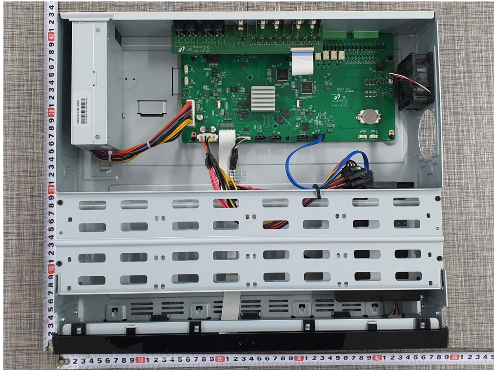
<Photo 9 > Internal view (HRX-835 model)
