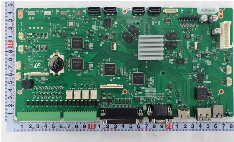
<Photo 13 > Component view (Main board - HRX-1632 model)
