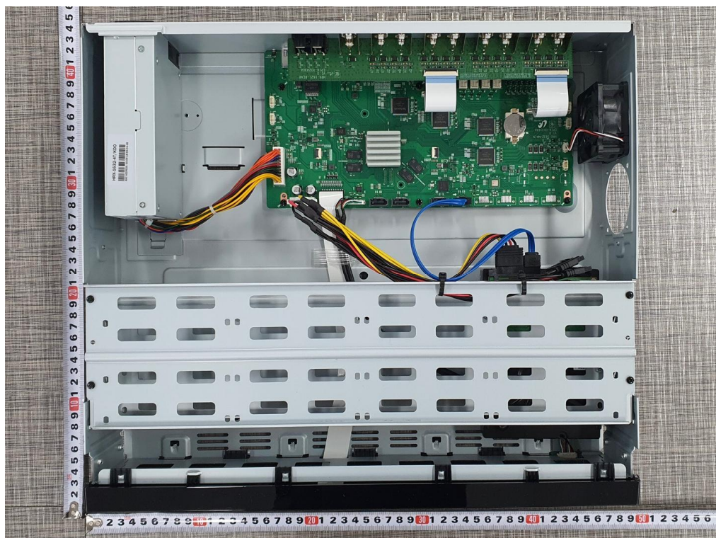
<Photo 8 > Internal view (HRX-1632 model)
