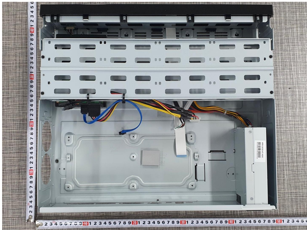
<Photo 10 > Internal view
