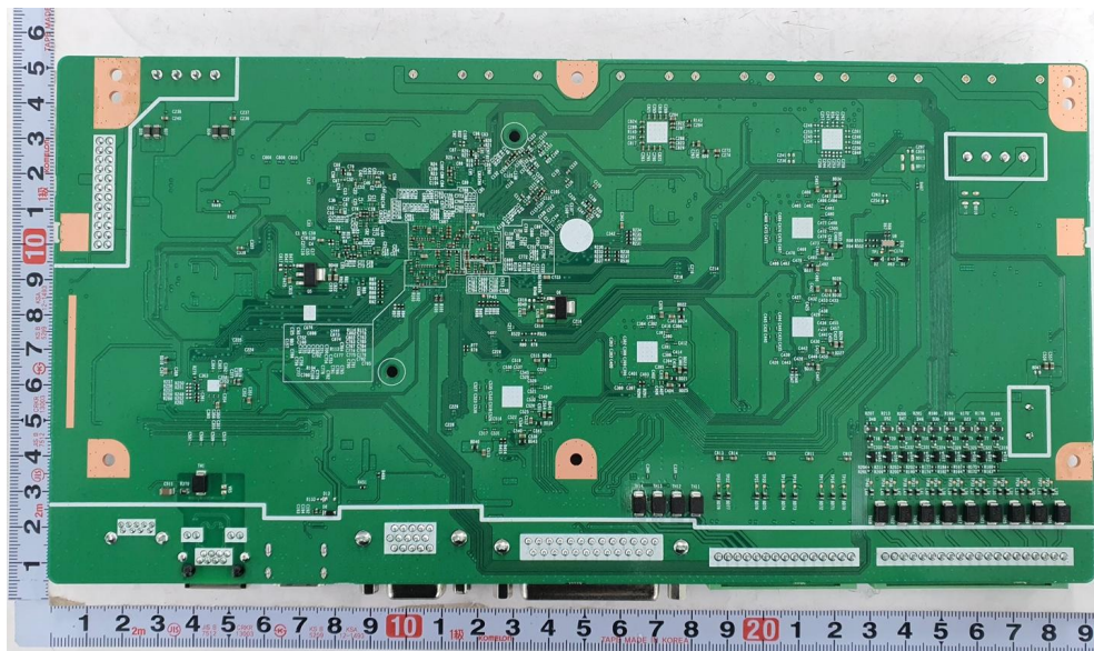
<Photo 14 > Soldering view (Main board - HRX-1632 model)
