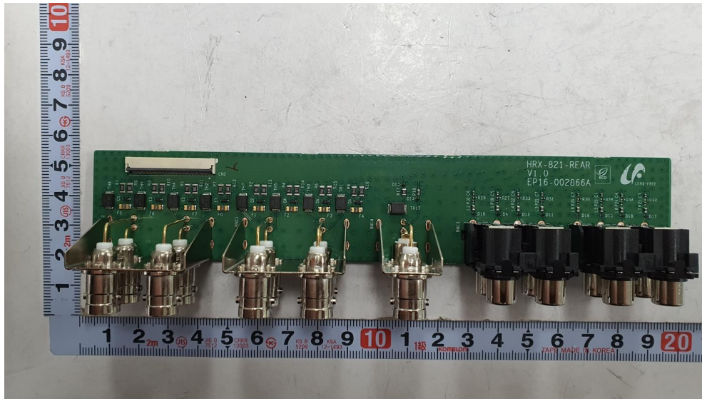
<Photo 19 > Component view (HRX-835 model)
