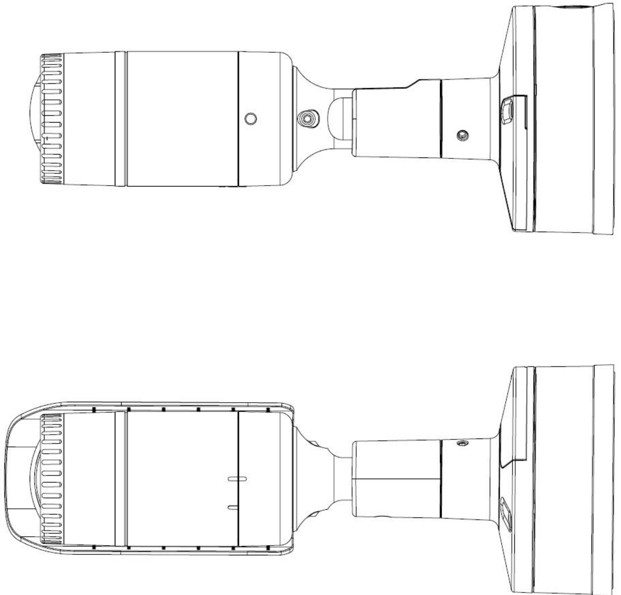
Appearance XNO-6010R Unit : mm [inch]
