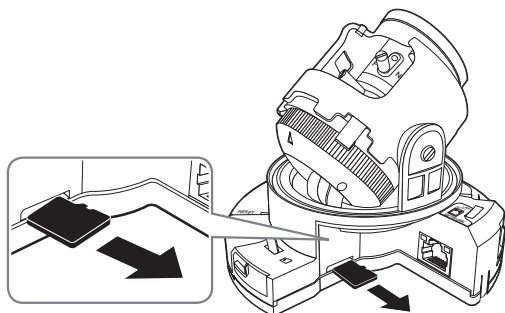
<LND-6012R/6022R/6032R/6072R>
