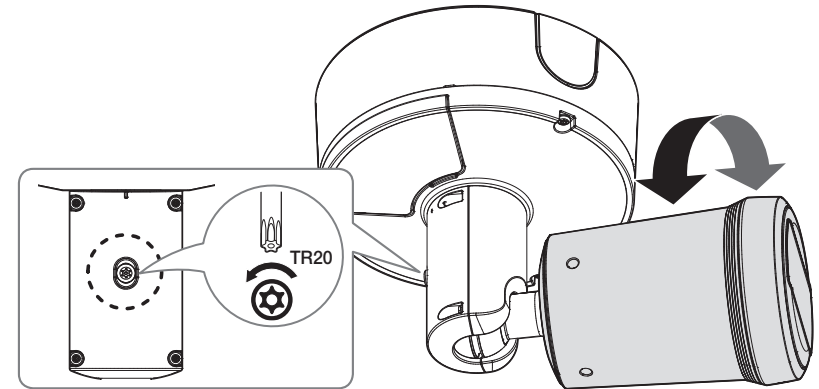
Lens rotation
