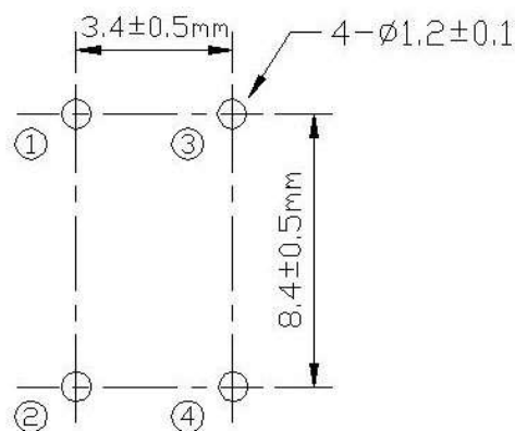
Minimum PCB Piercing HOLE
