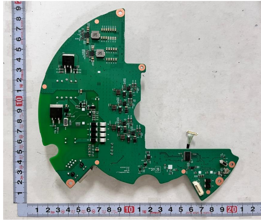
<Photo 8> Main board view 1
