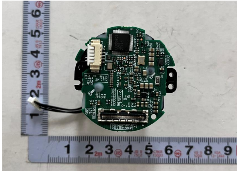
<Photo 17> Camera module view 4
