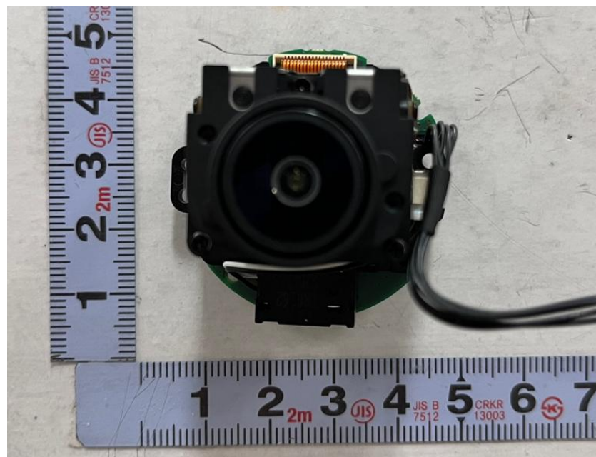
<Photo 16> Camera module view 3
