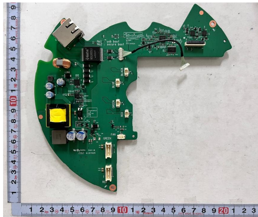
<Photo 6> Network board view 1
