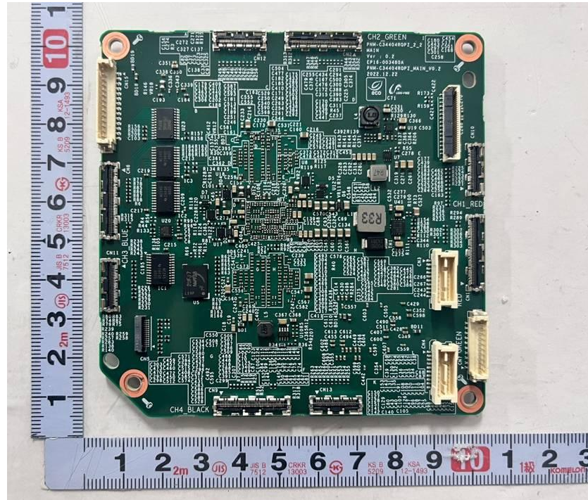
<Photo 22> Main board view 2
