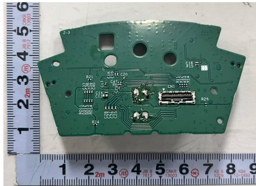
<Photo 20> Interface board view 2
