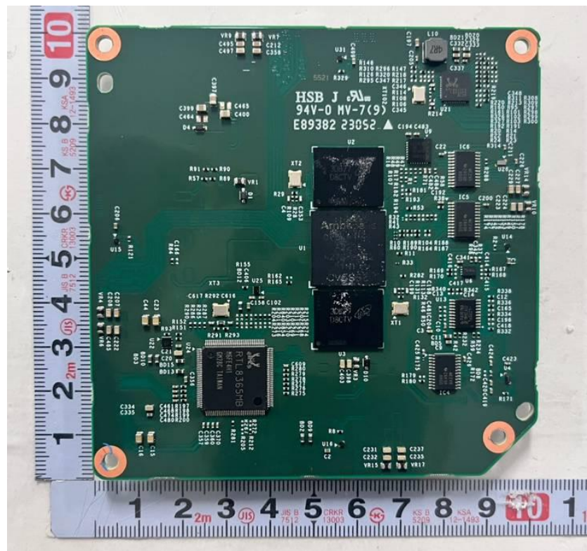
<Photo 22> Main board view 2
