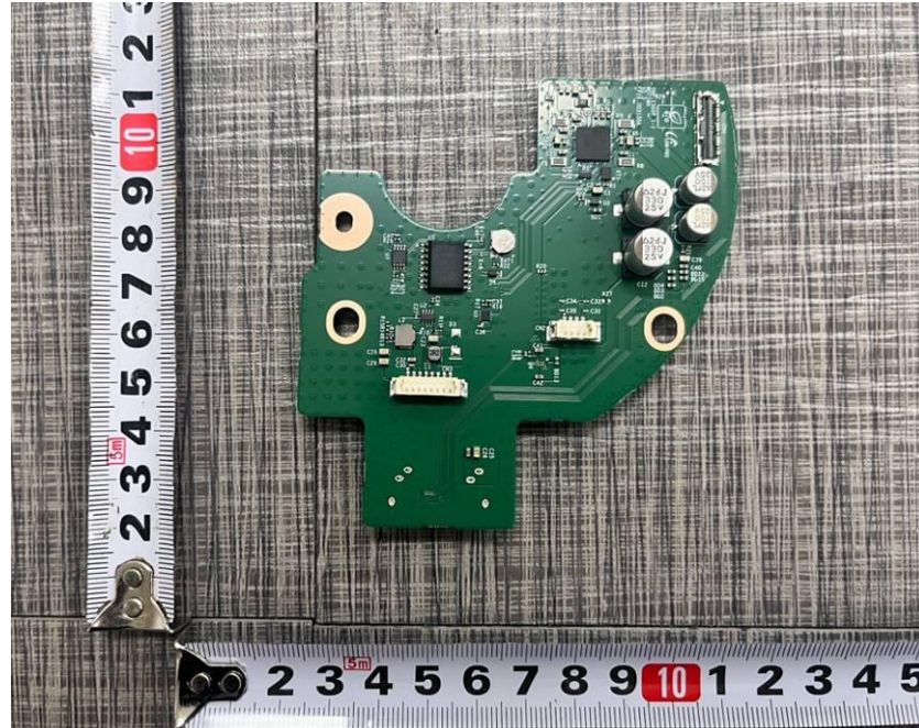
<Photo 14> Drive board view 2
