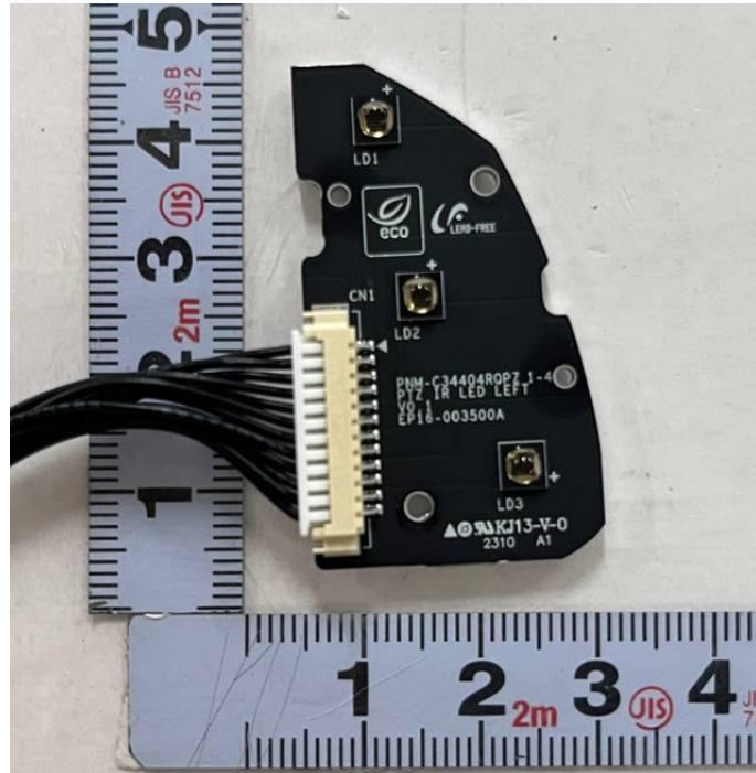
<Photo 34> PTZ LED board view 2
