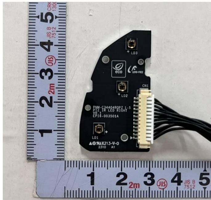
<Photo 34> PTZ LED board view 2
