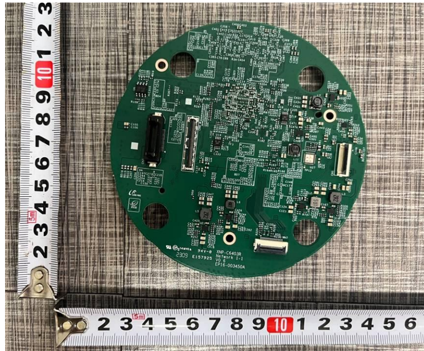
<Photo 26> Network board view 2
