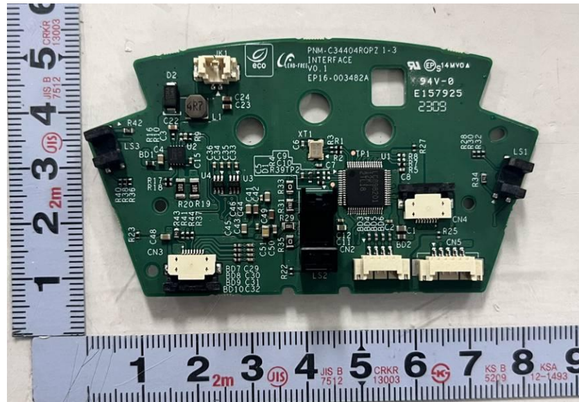
<Photo 20> Interface board view 2
