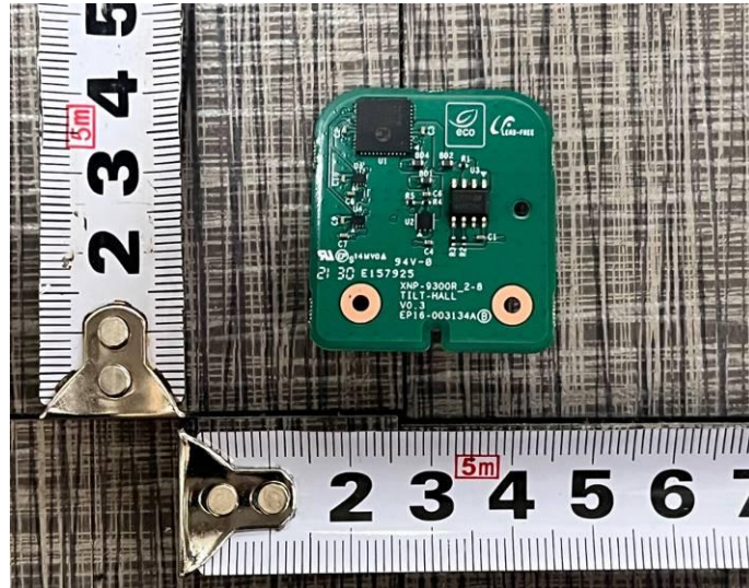
<Photo 44> Tilt hall board view 2
