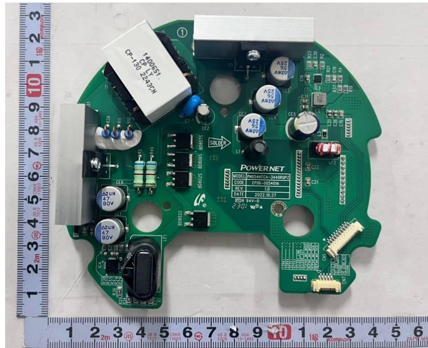
<Photo 28> Power board view 2
