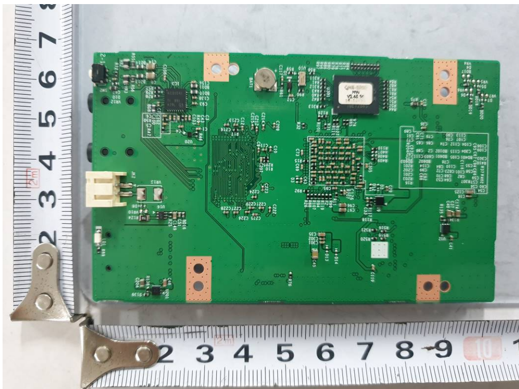
< Photo 6 > Main board bottom view
