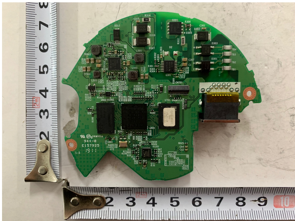
<Photo 6> Network board 후면
