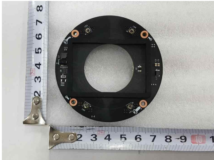
<Photo 9> LED board 전면
