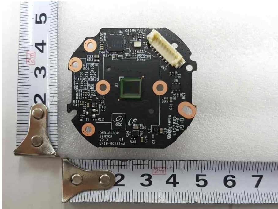
<Photo 7> Sensor board 전면
