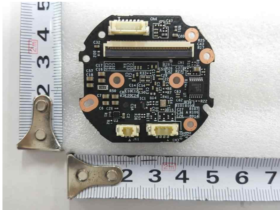
<Photo 8> Sensor board 후면
