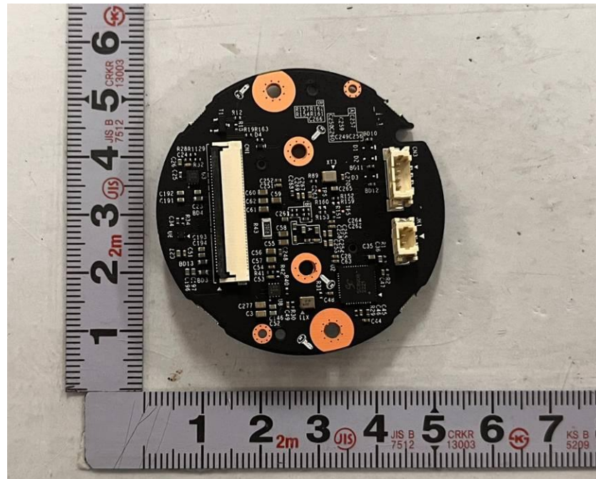
<Photo 14> Network board view 1
