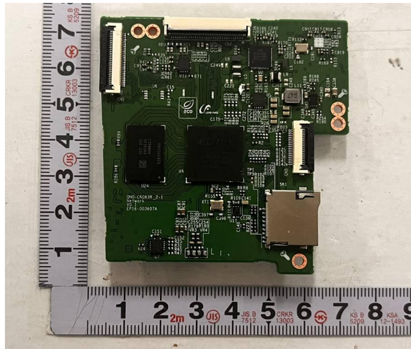
<Photo 14> Network board view 1
