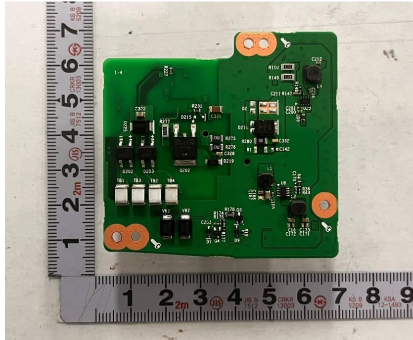
<Photo 17> Power board view 2
