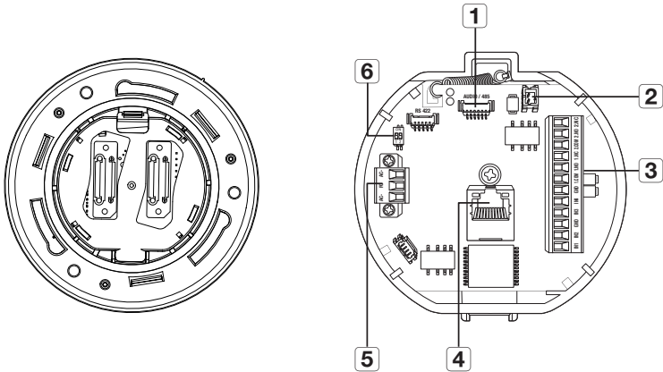
Bottom View of Installation Base
