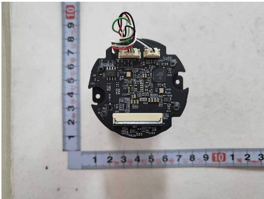
<Photo 8> Sensor Board
