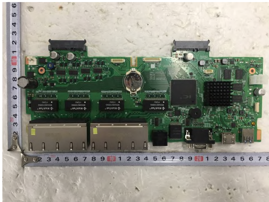
&lt;Photo 4 &gt; Main board Top view
