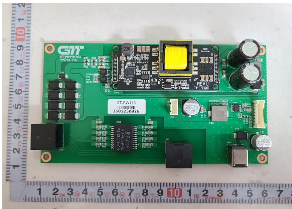
<Photo 4>Power board
