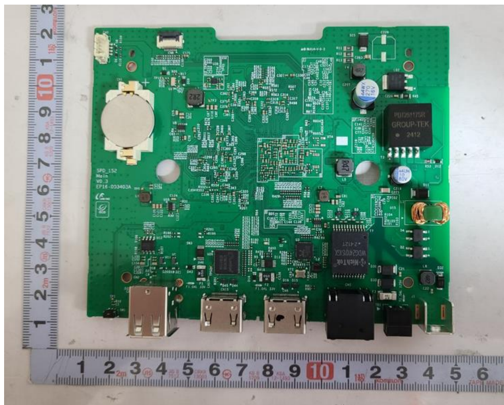
&lt;Photo 10&gt; Video decoder board
