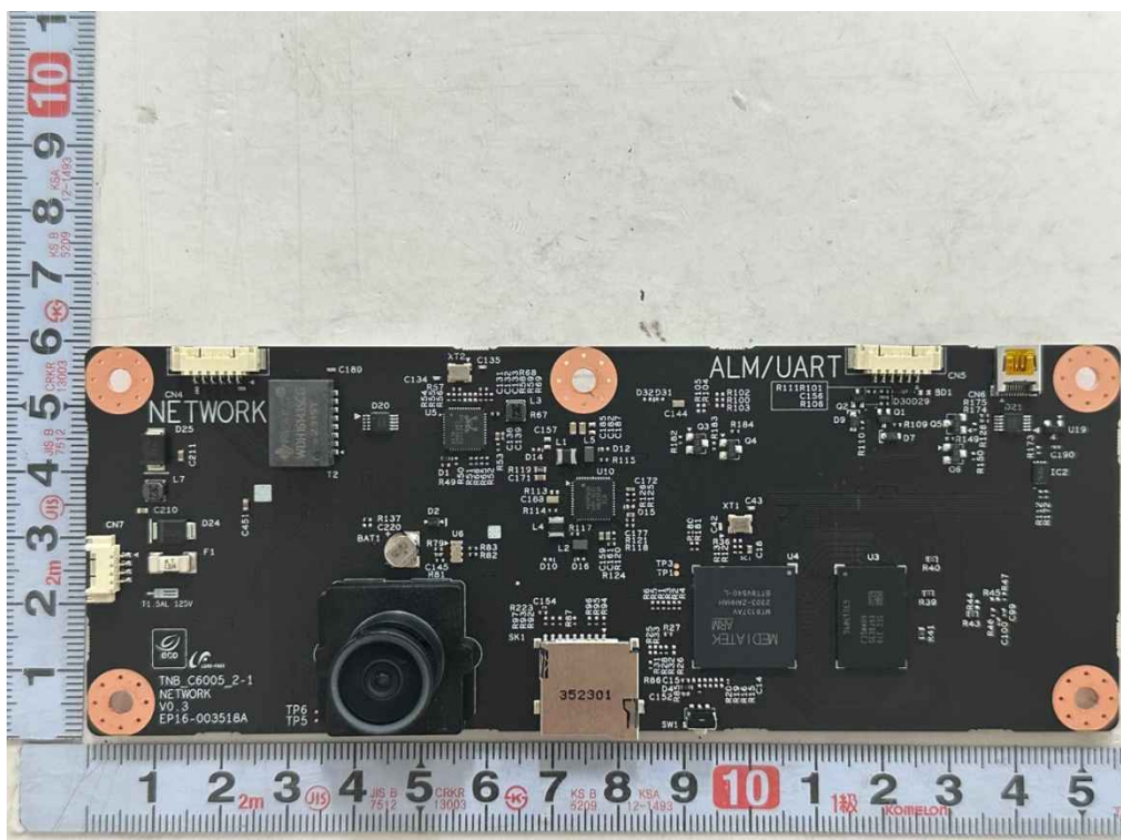
<Photo 4 > Network Camera board
