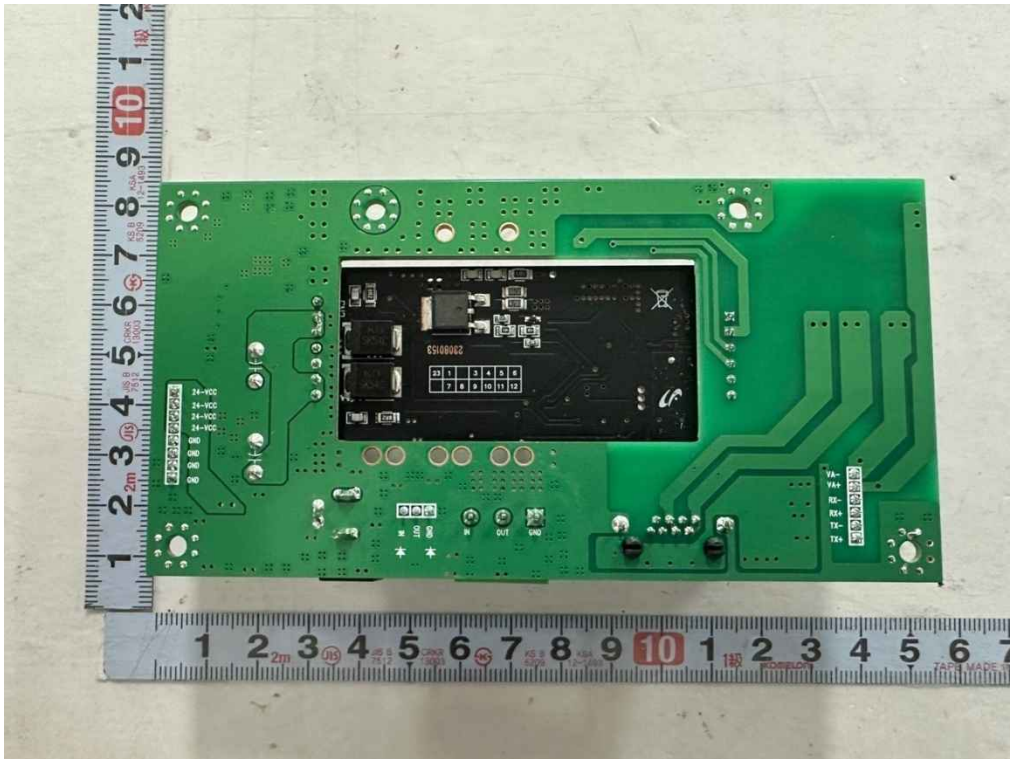
<Photo 7 > PoE board
