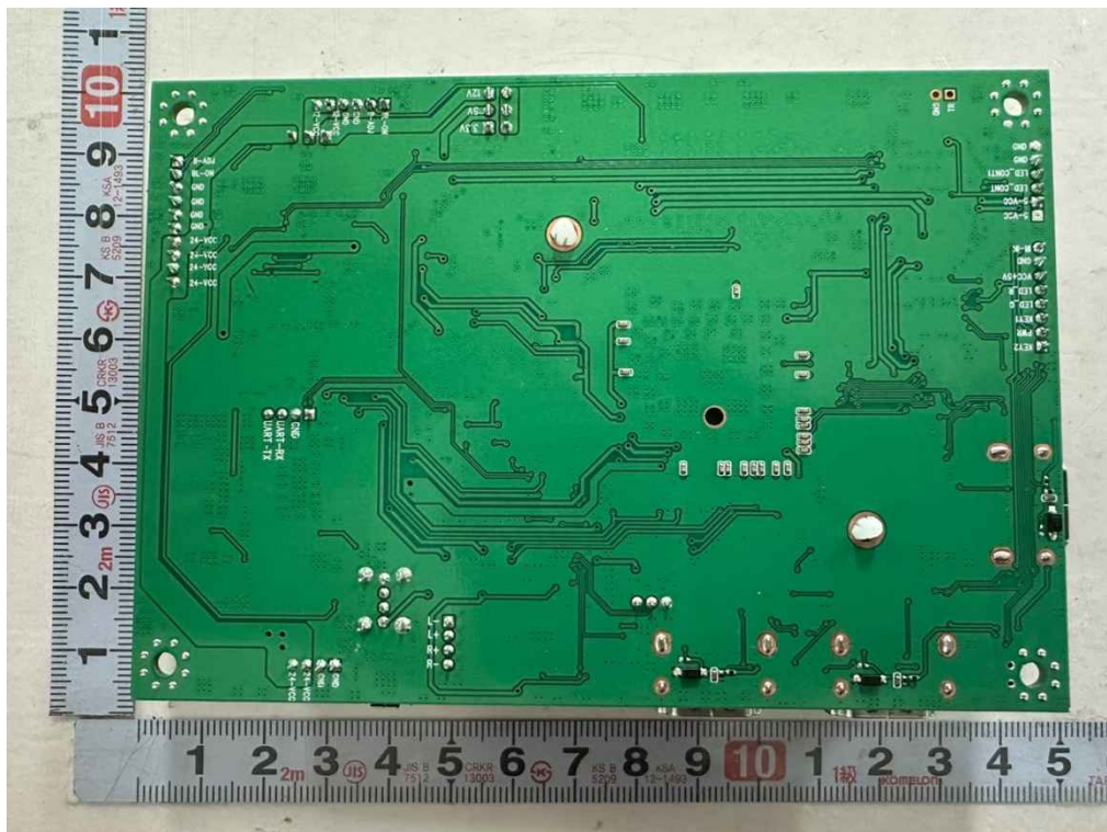
<Photo 9 > RMM411 board
