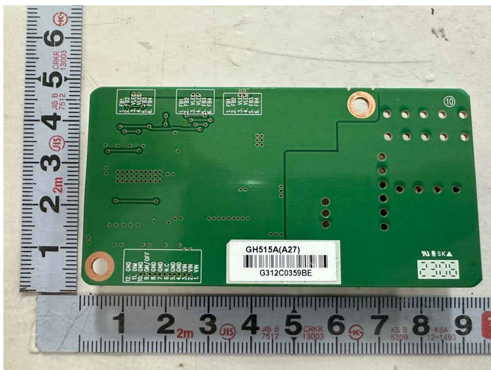
<Photo 11 > LED driver board
