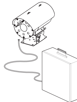
<Standard method to install camera and washer pump>
