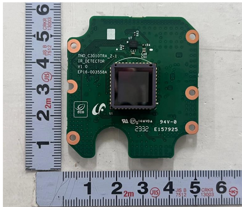
<Photo 16> IR_DETECTOR view 2
