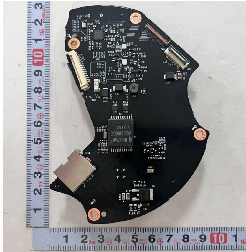
<Photo 8> Network board view 1
