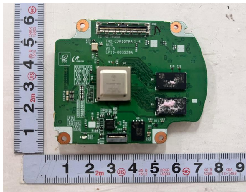
<Photo 10> NUC board view 1
