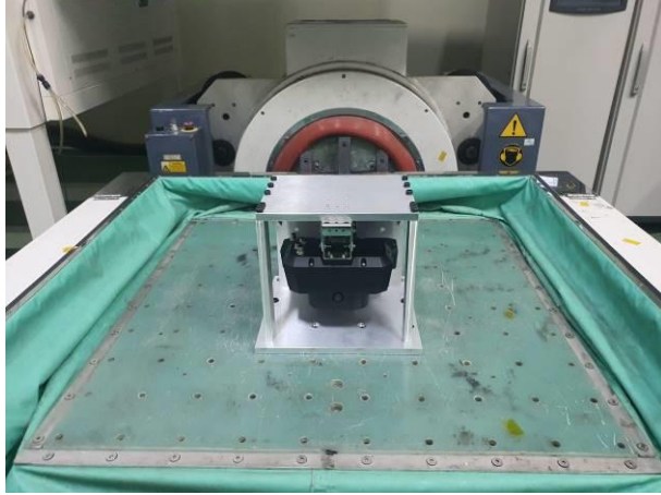
Vibration(Sine) Test[IEC/EN 60068-2-6:2007] – X axis, Test Shock(impact) Test Same configuration
