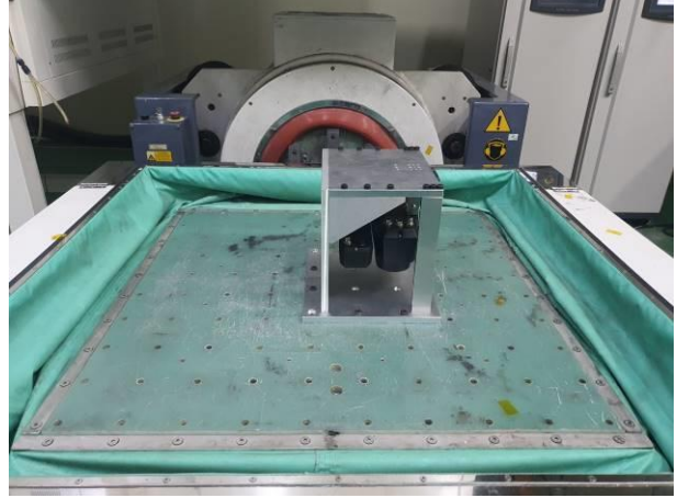
Vibration(Sine) Test[IEC/EN 60068-2-6:2007] – Y axis, Test Shock(impact) Test Same configuration
