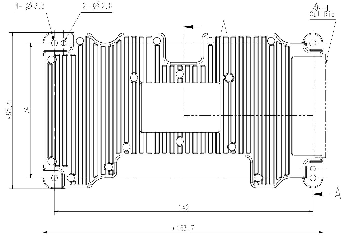
STANDARD TOLERANCE
