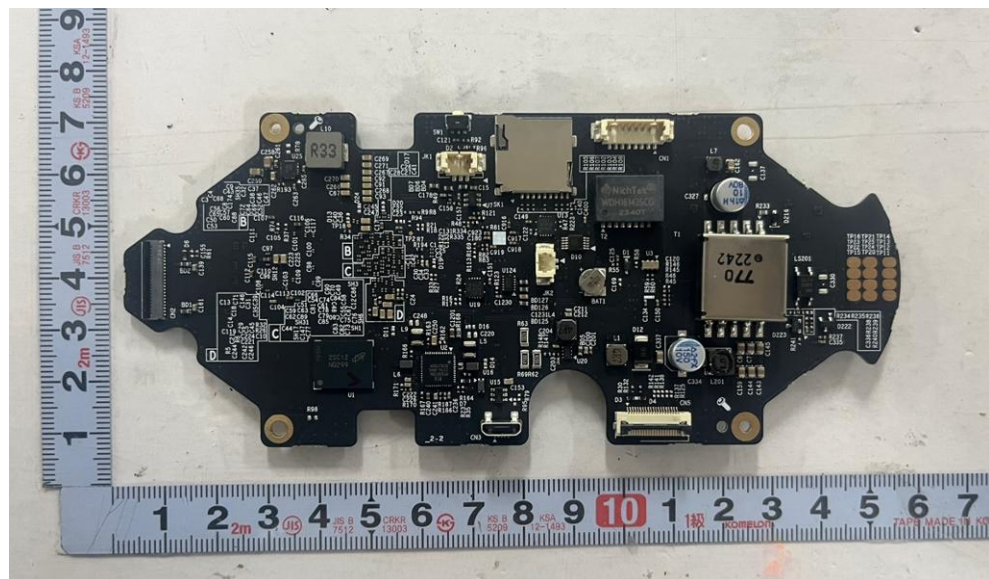
<Photo 12> Network board 2
