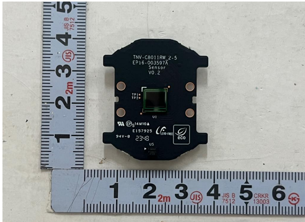
<Photo 10> Sensor board 2
