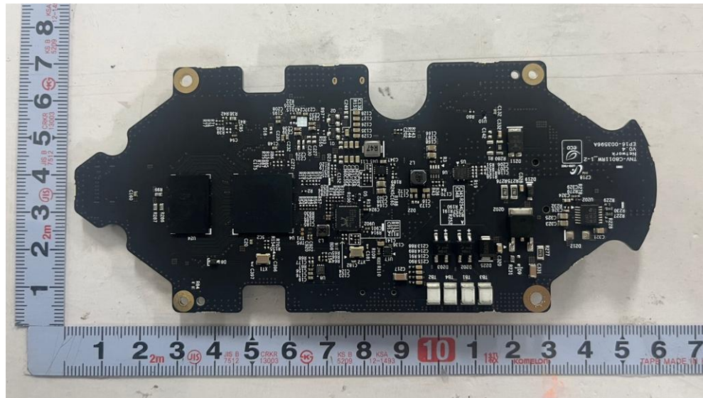
<Photo 12> Network board 2
