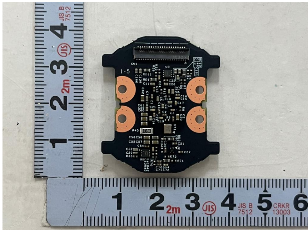
<Photo 10> Sensor board 2
