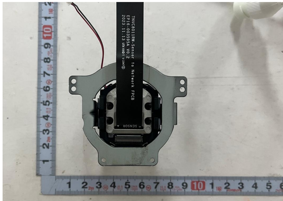
<Photo 8> Camera module 2
