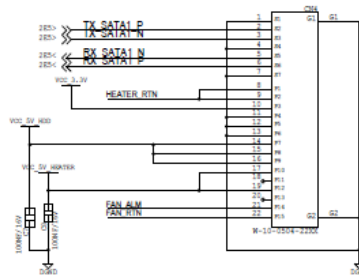
BOTTOM BACKPLANE TO SATA #2
