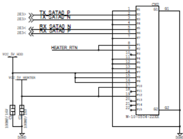
TOP BACKPLANE TO SATA #1
