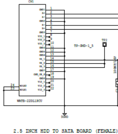
HDD TO SATA BOARD
