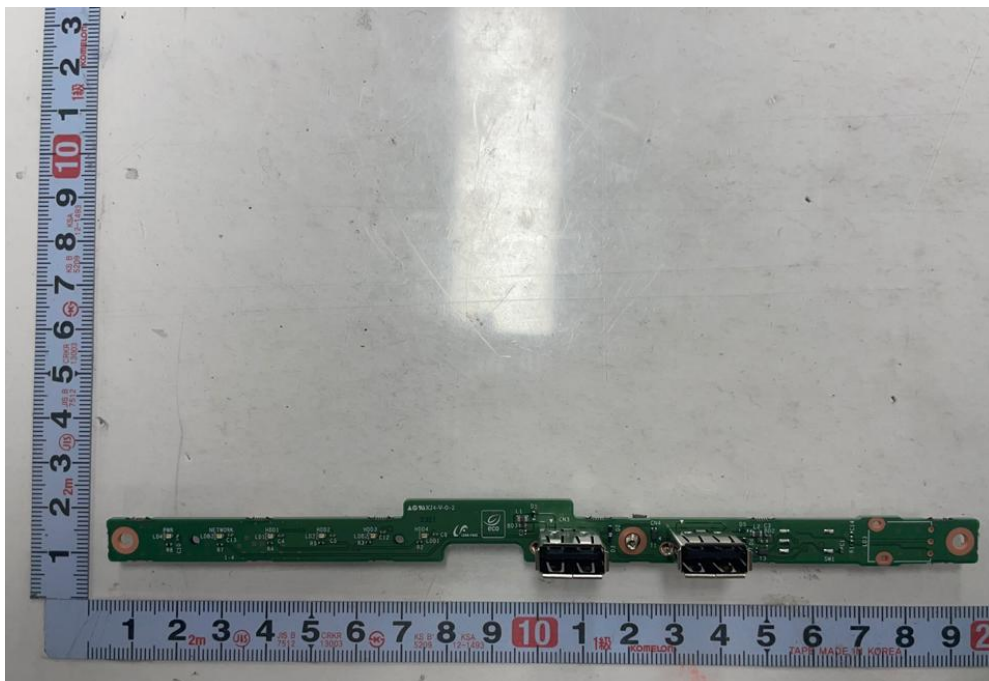
<Photo 10 > Front USB board view
