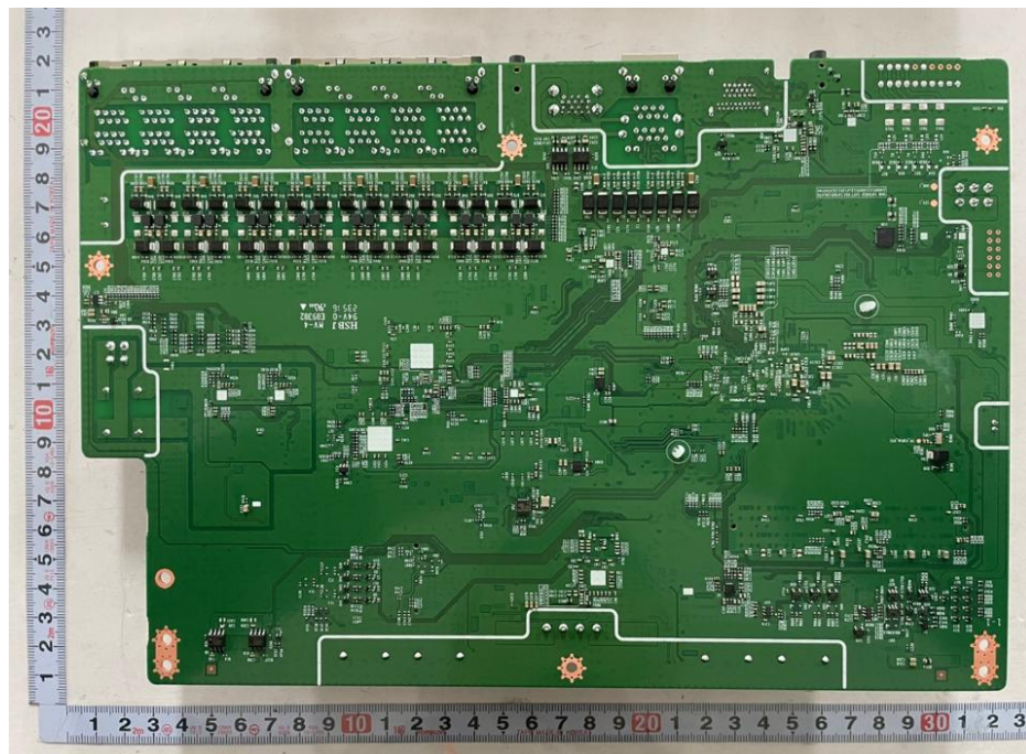
<Photo 9 > Mainboard bottom view
