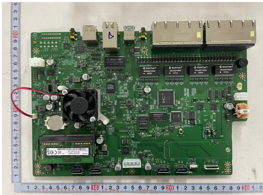
<Photo 8 > Mainboard top view
