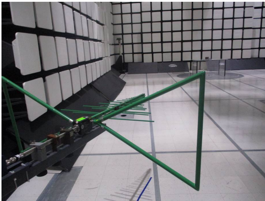
Figure 6. RE (30 MHz – 1 GHz) Test Setup, Antenna View
