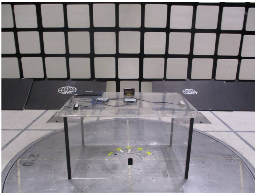
Figure 7. RE (30 MHz – 1 GHz) Test Setup, Front View
