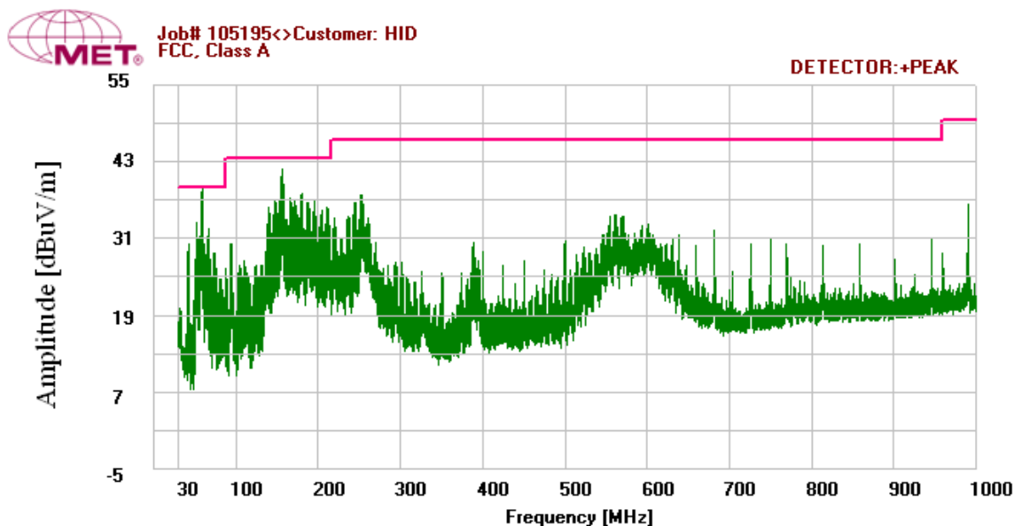
Figure 5. RE FCC - (30 MHz – 10 GHz), Plot
