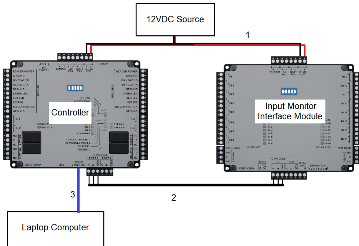
Figure 2. Block Diagram of Test Configuration
