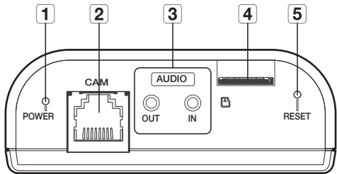
Front of the main unit
