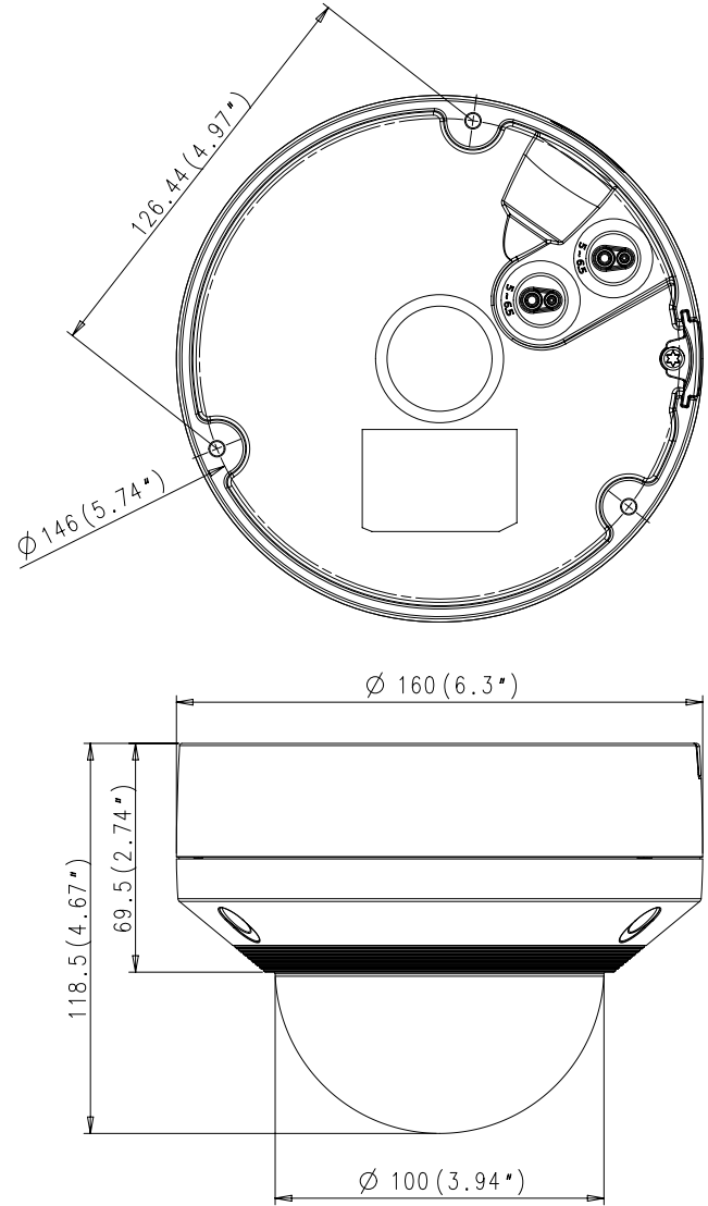
XNV-6080/6080R/8080R
