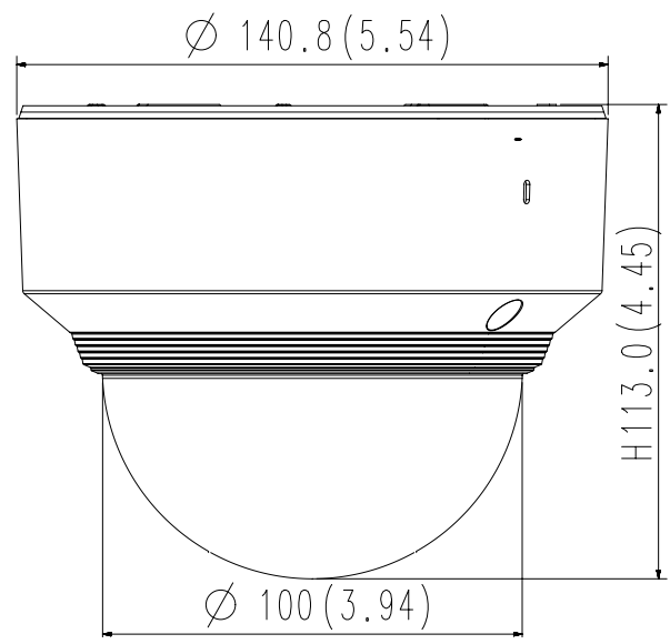
XND-6080V/6080RV/8080RV
