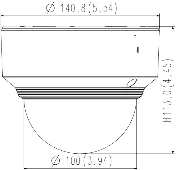
XND-6080V/6080RV/8080RV
