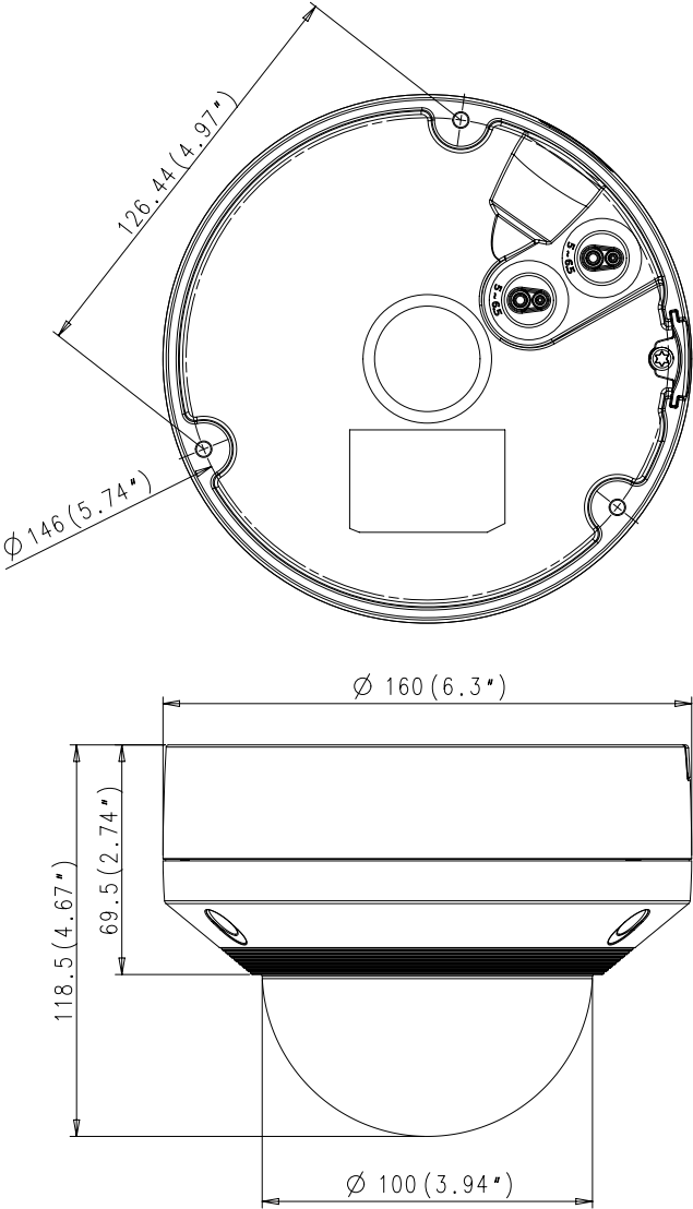
XNV-6080/6080R/8080R
