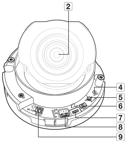
<XND-6080V>
