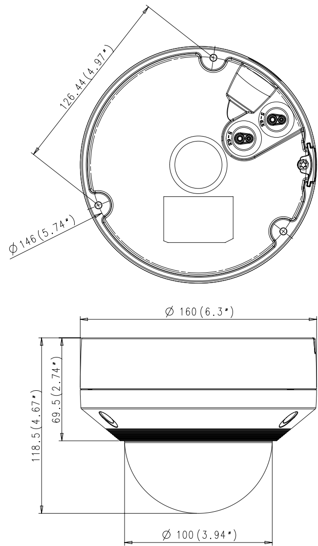
XNV-6080/6080R/8080R
