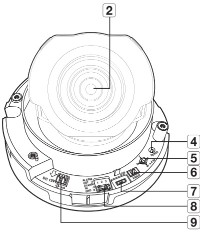
<XND-6080V>
