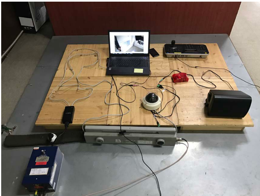
Conducted Disturbances, Induced by Radio-Frequency Fields / Capture mode (PoE)
