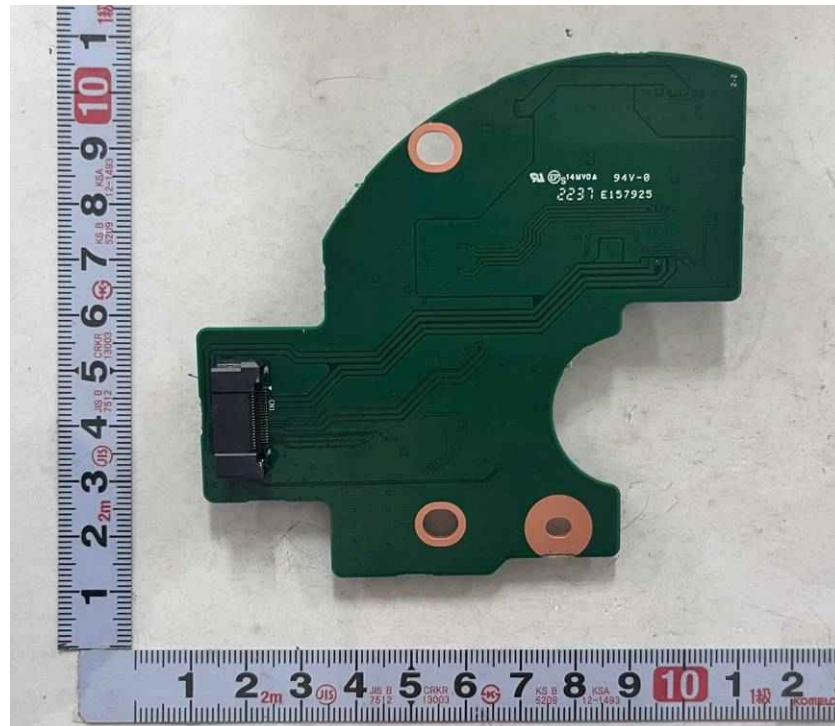
<Photo 24> Network board top view
