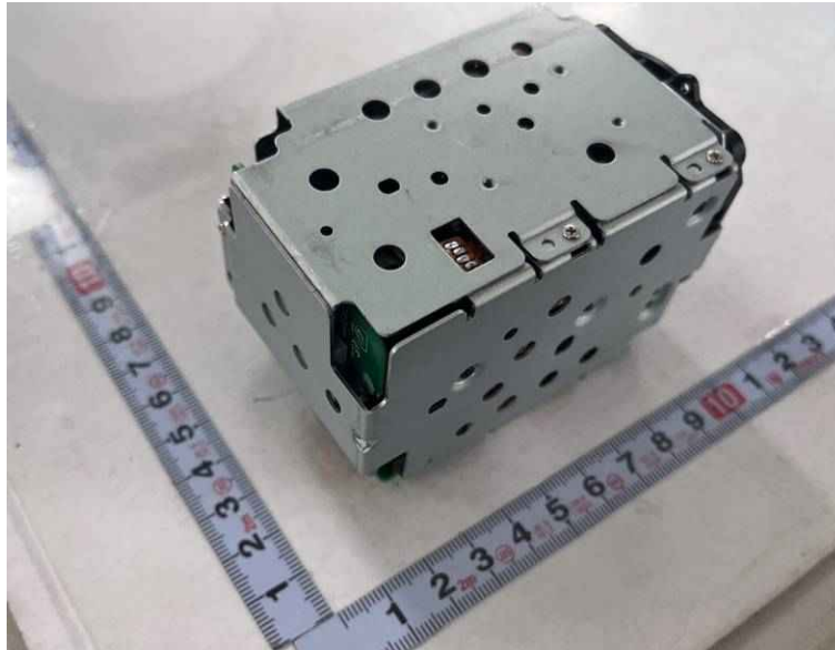
<Photo 14> Sensor board view
