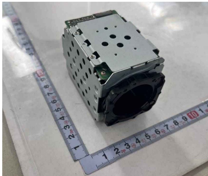
<Photo 12> Camera module view 1
