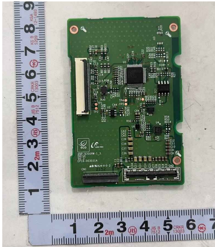
<Photo 16> Drive board bottom view
