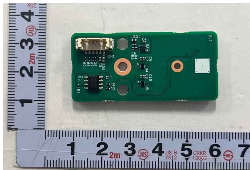
<Photo 30> Hall board top view
