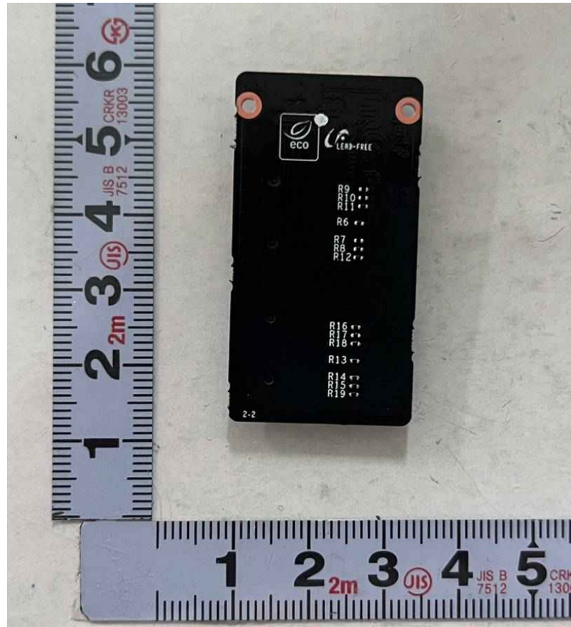
<Photo 18> Micro SD board bottom view
