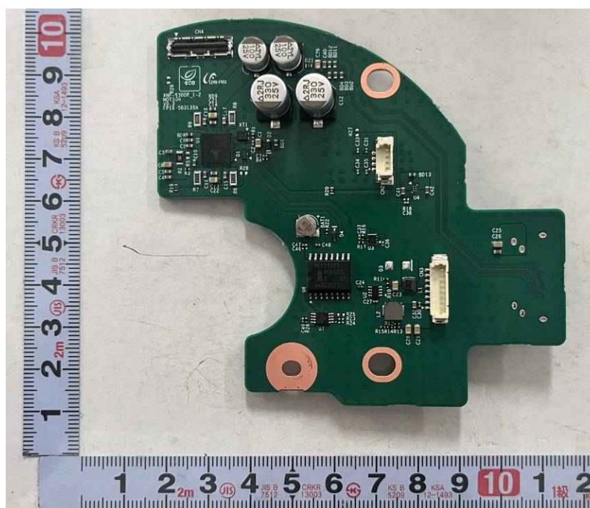
<Photo 22> Motion board top view
