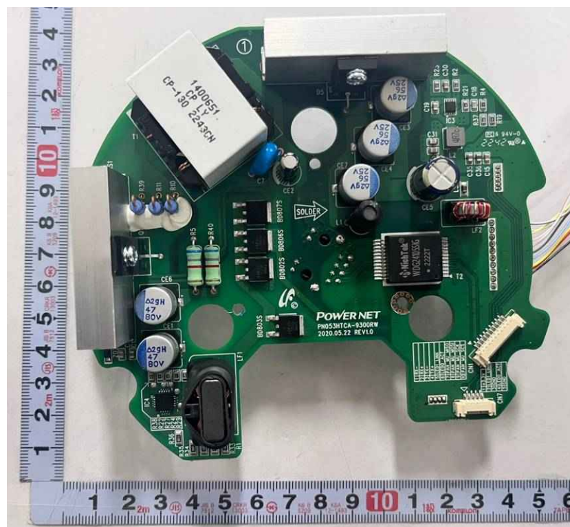
<Photo 28> Power board top view
