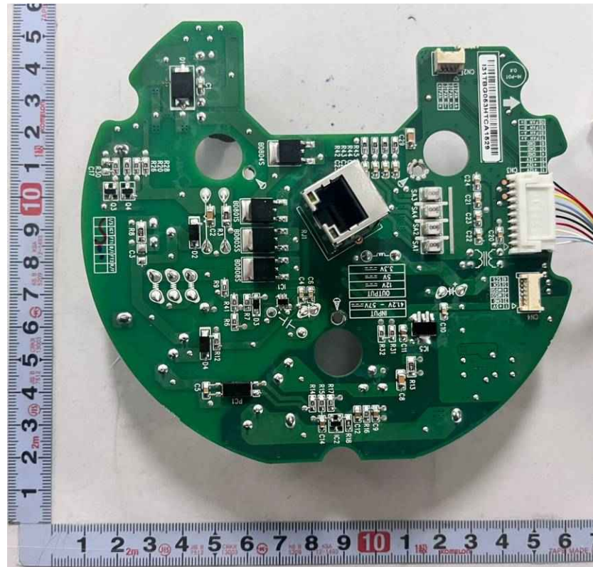
<Photo 30> Hall board top view
