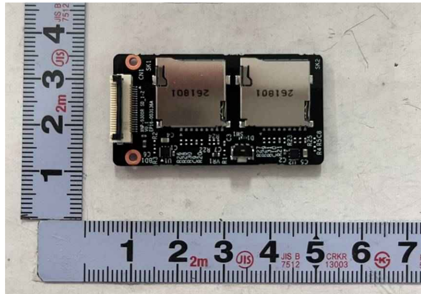
<Photo 18> Micro SD board bottom view
