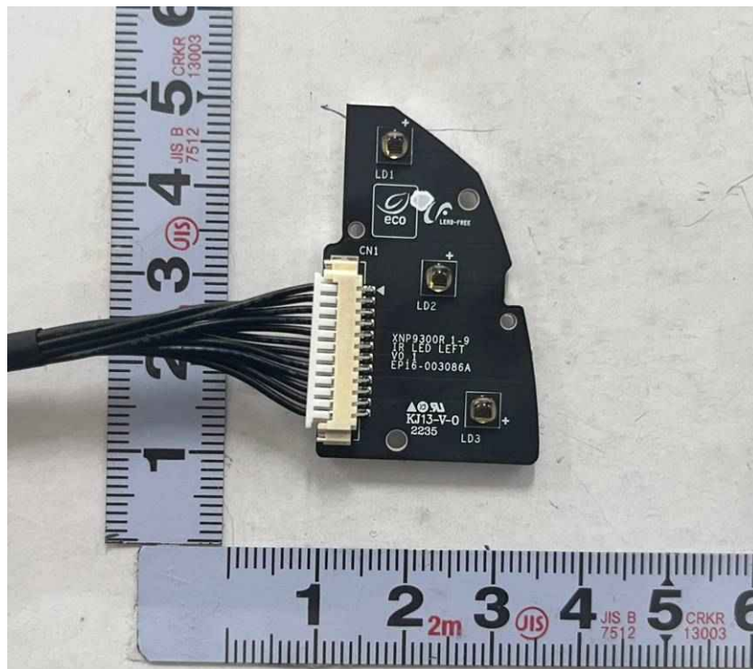
<Photo 20> LED board view left
