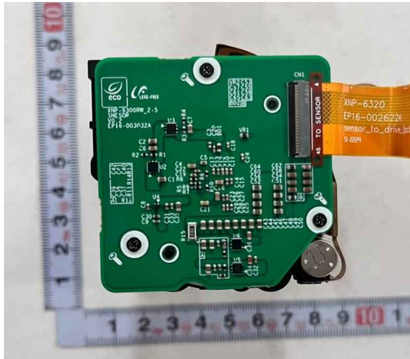
<Photo 14> Sensor board view
