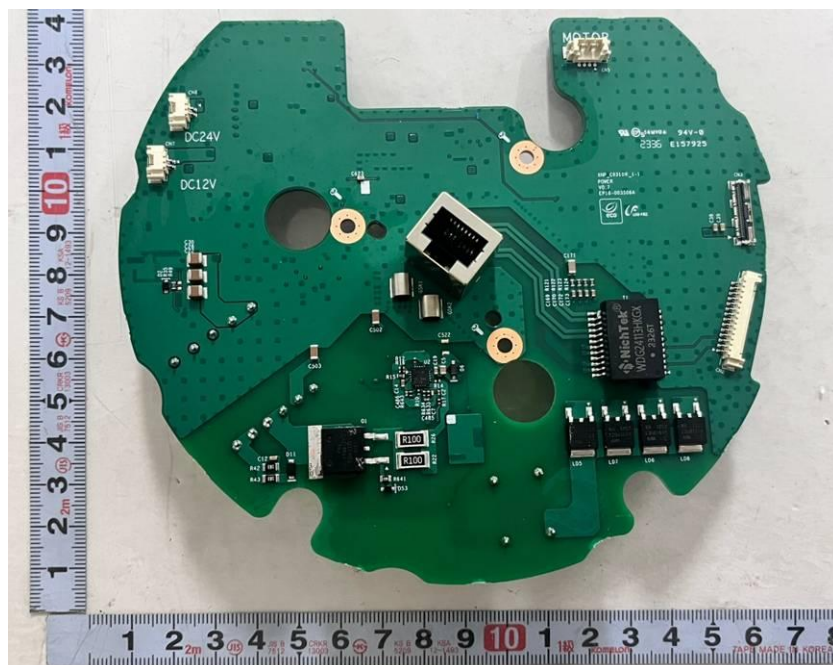
<Photo 26> Power board view 1
