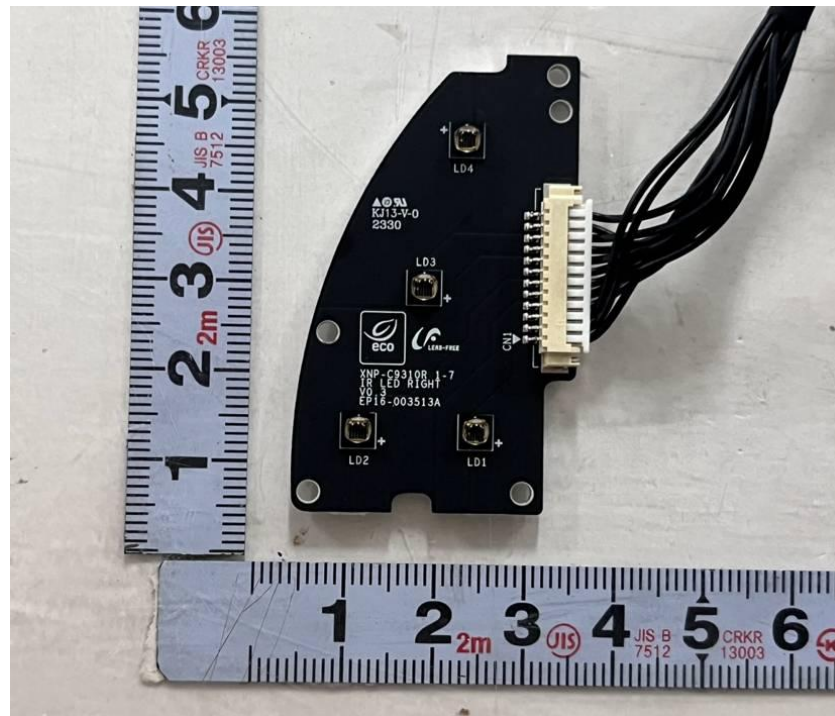
<Photo 20> IR LED right view
