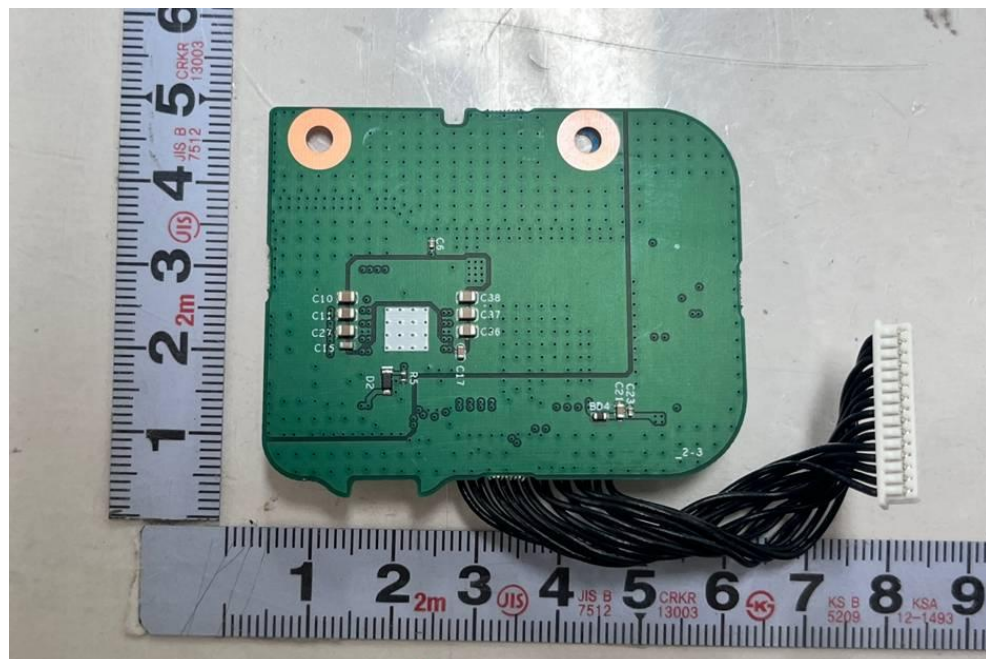
<Photo 10> Motion board view 2
