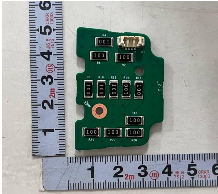
<Photo 18> Heater board view 2
