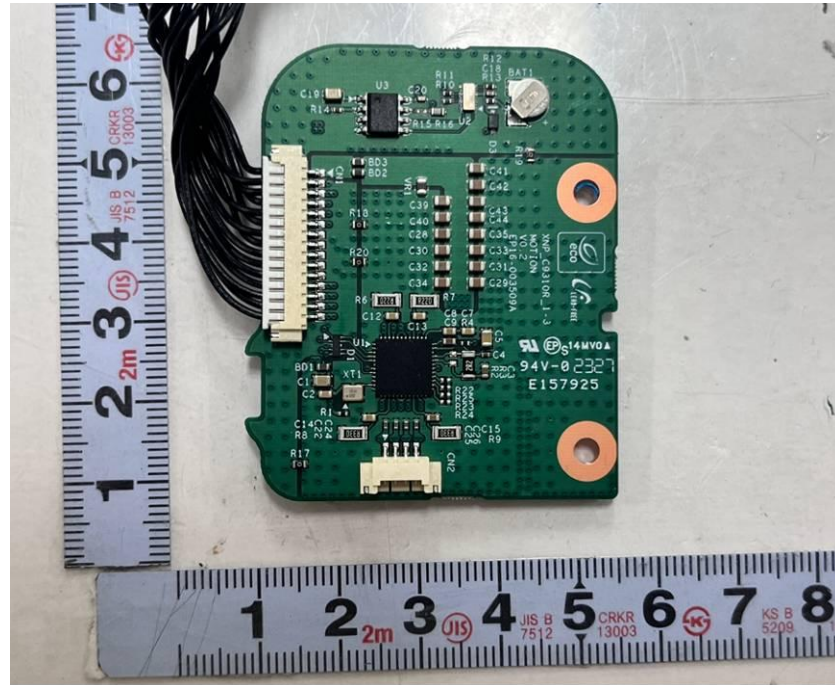
<Photo 10> Motion board view 2
