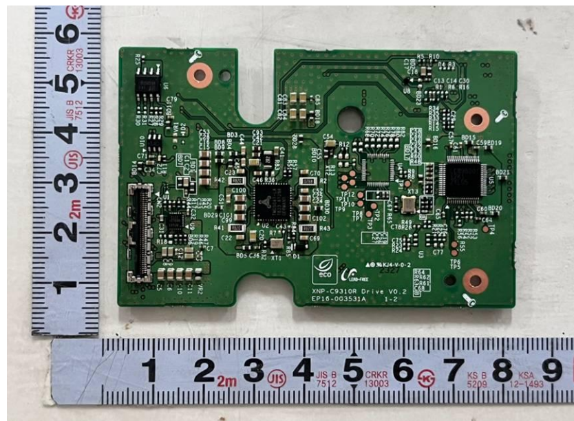
<Photo 22> Drive board view 1
