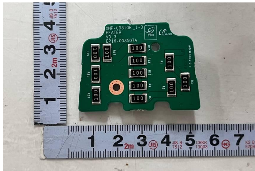
<Photo 18> Heater board view 2
