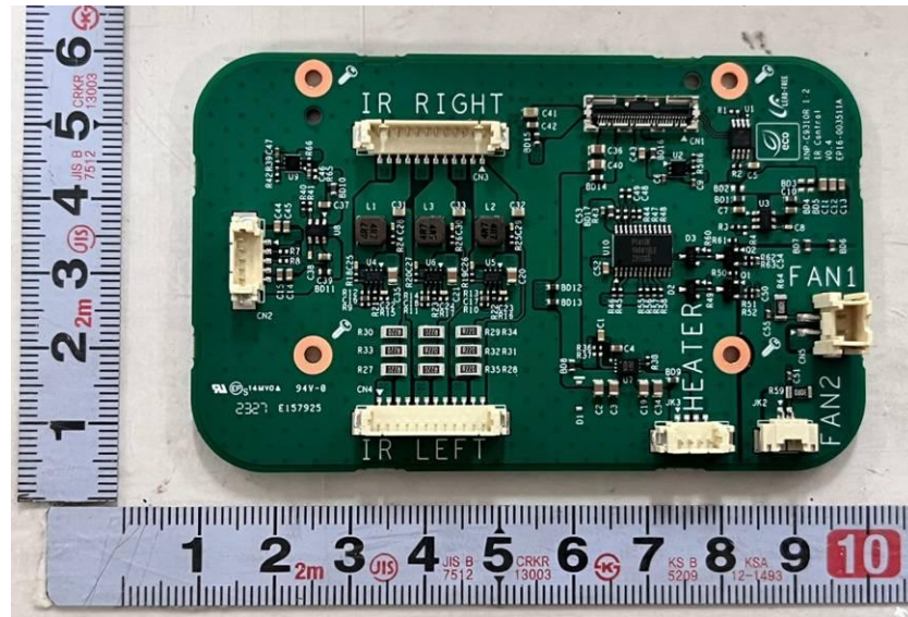
<Photo 22> Drive board view 1
