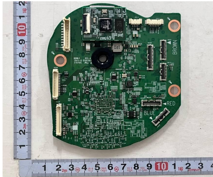
<Photo 12> Network board view 2
