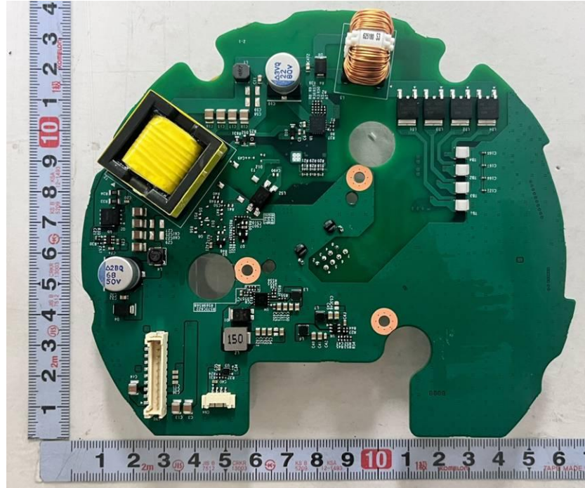
<Photo 27> Power board view 2
