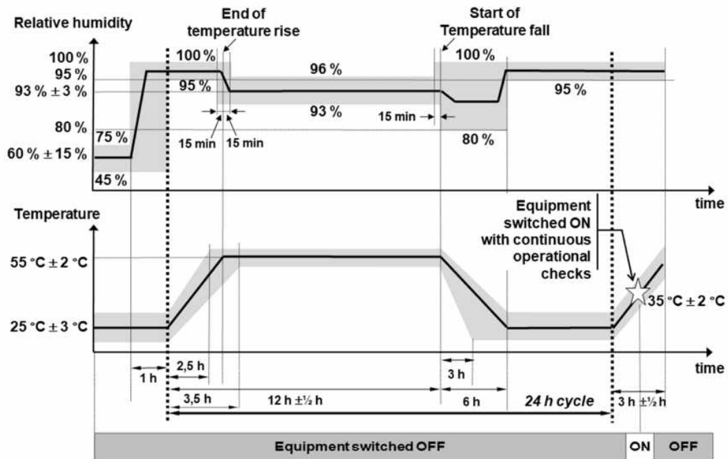
Figure 1 - Cyclic damp heat test: 1 st and begin of 2 nd 24-h cycle
