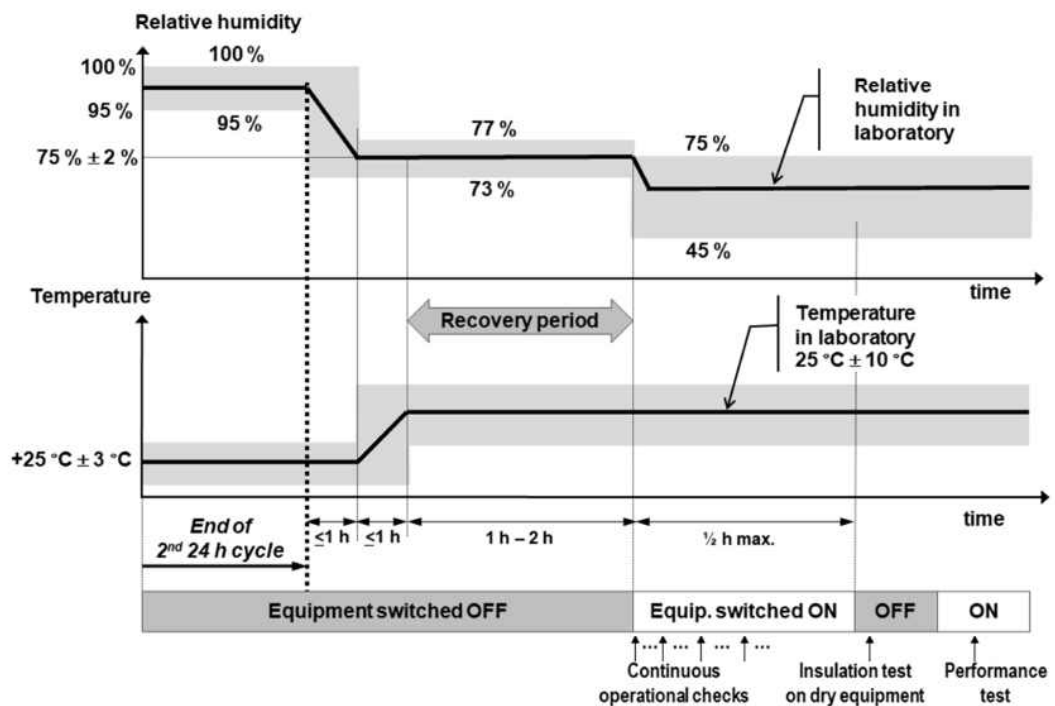
Figure 2 - Cyclic damp heat test: End of 2 nd cycle and recovery period
