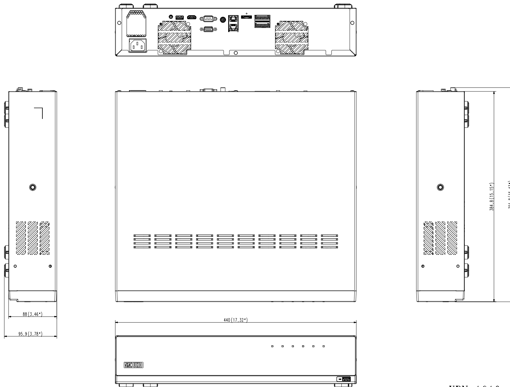
XRN-1610 Appearance drawing
