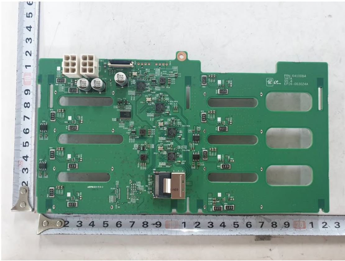
<Photo 10 > HDD board view (Bottom)
