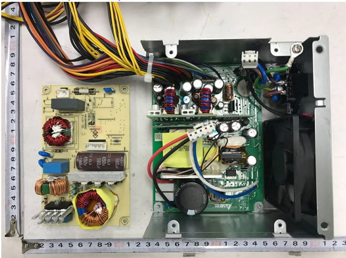
<Photo 6 > Internal view (SMPS board)
