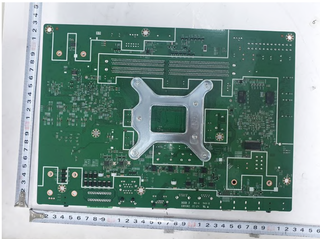
<Photo 8 > Main board view (Bottom)
