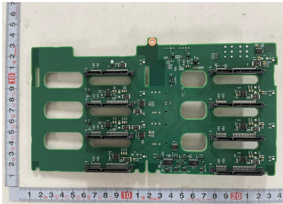
&lt;Photo 13 &gt; SATA-L board view
