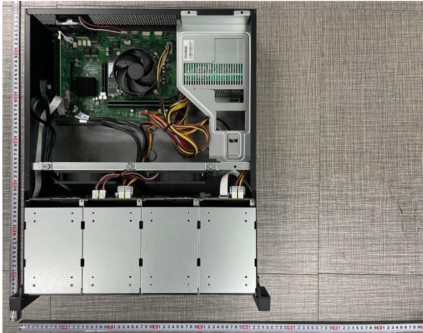
<Photo 5 > Internal view
