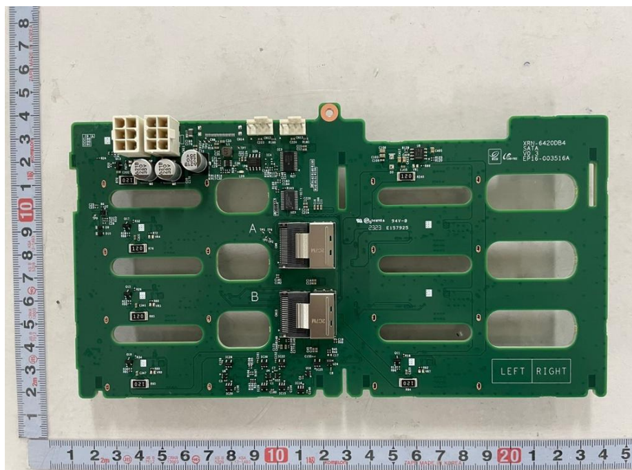
&lt;Photo 12 &gt; SATA-L board view
