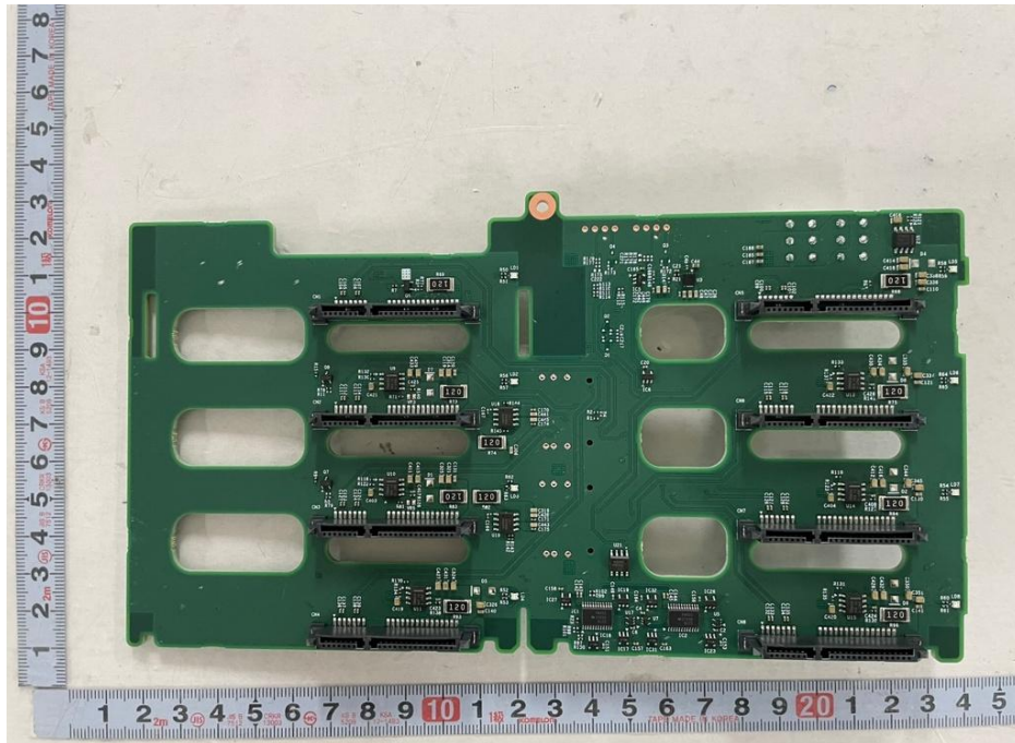
&lt;Photo 15 &gt; SATA-R board view
