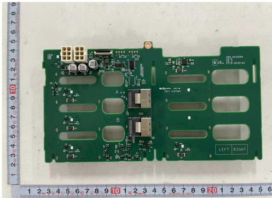
&lt;Photo 14 &gt; SATA-R board view
