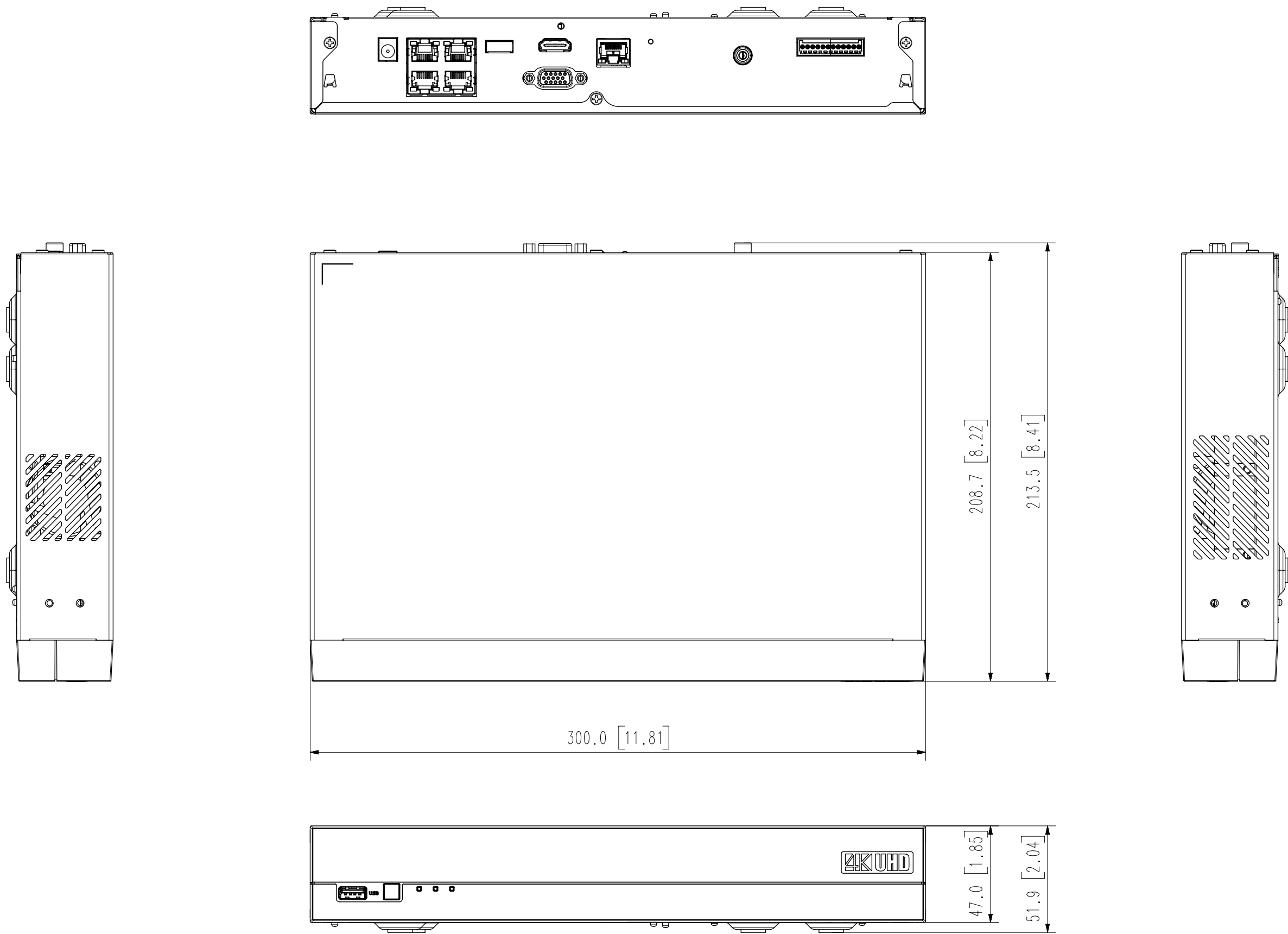
Appearance Drawing XRN-410S Unit : mm[inch]
