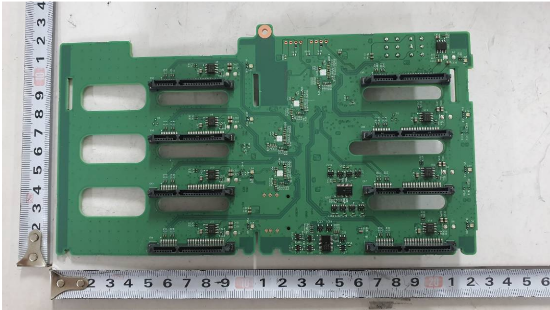
<Photo 9 > HDD board (Bottom)
