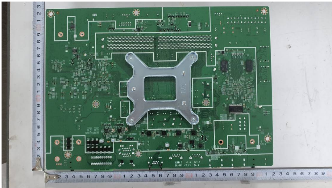
<Photo 7 > Main board (Bottom)
