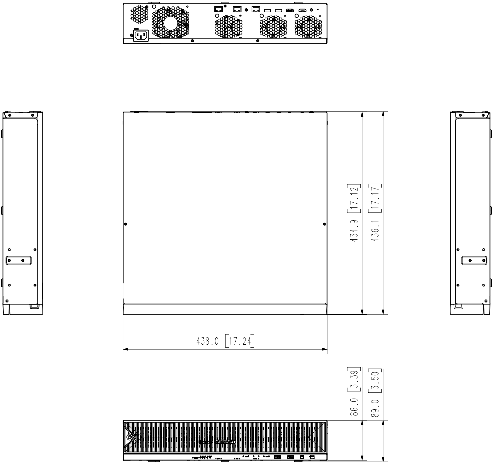
Appearance Drawing XRP-4010B2 Unit : mm [inches]
