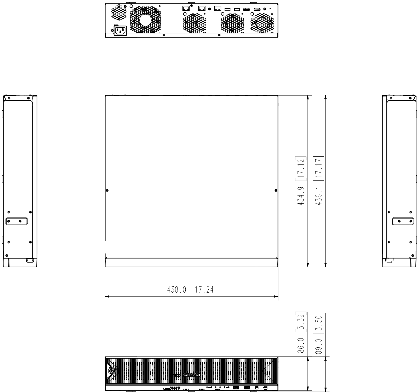
Appearance Drawing XRP-4110B2 Unit : mm [inches]
