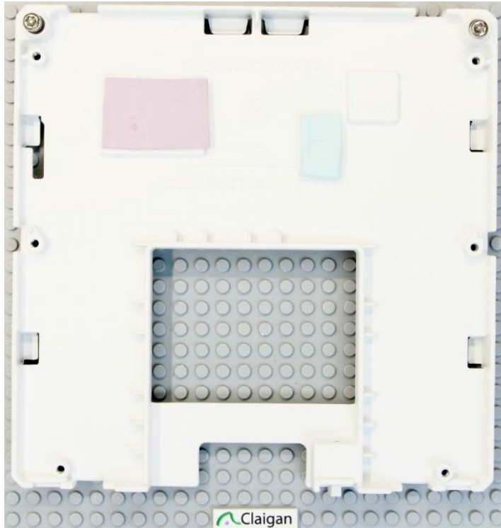
119798 Exploded view
