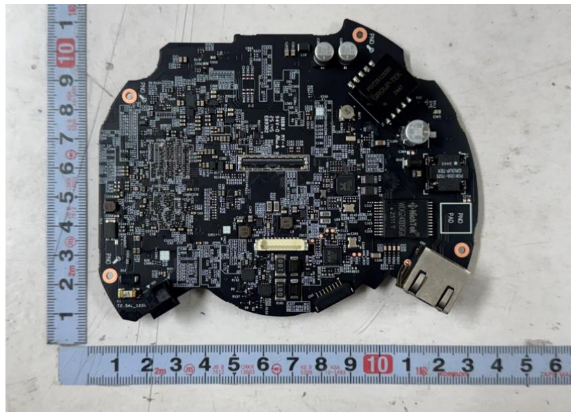
<Photo 10> Network board view 2
