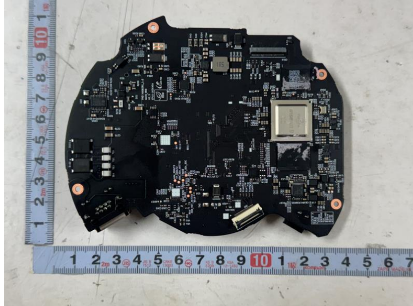
<Photo 10> Network board view 2
