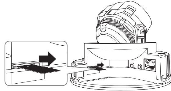
<PND-9080R>
