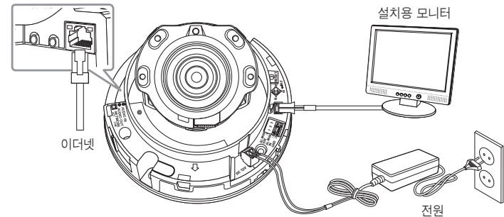
<PND-9080R>
