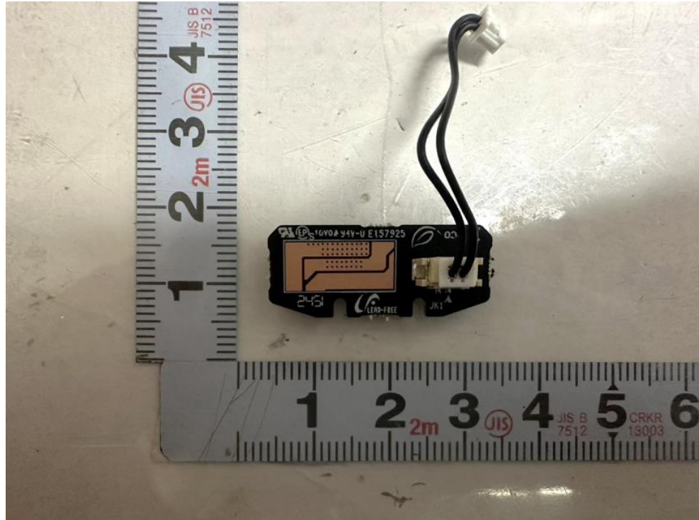
<Photo 17> IR LED board view 4
