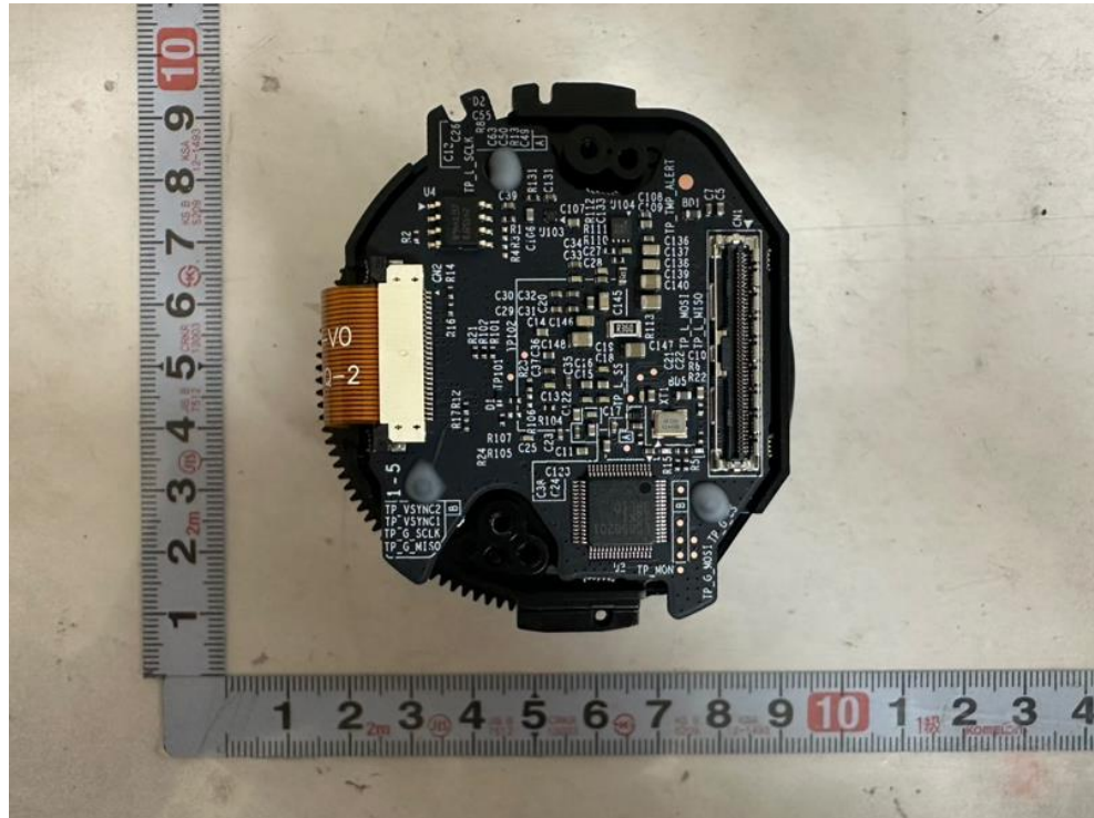
<Photo 12> Heater board view 1
