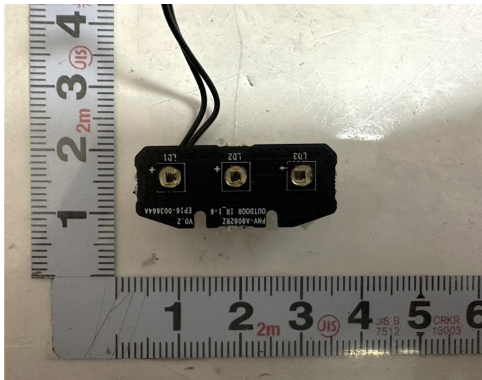
<Photo 16> IR LED board view 3
