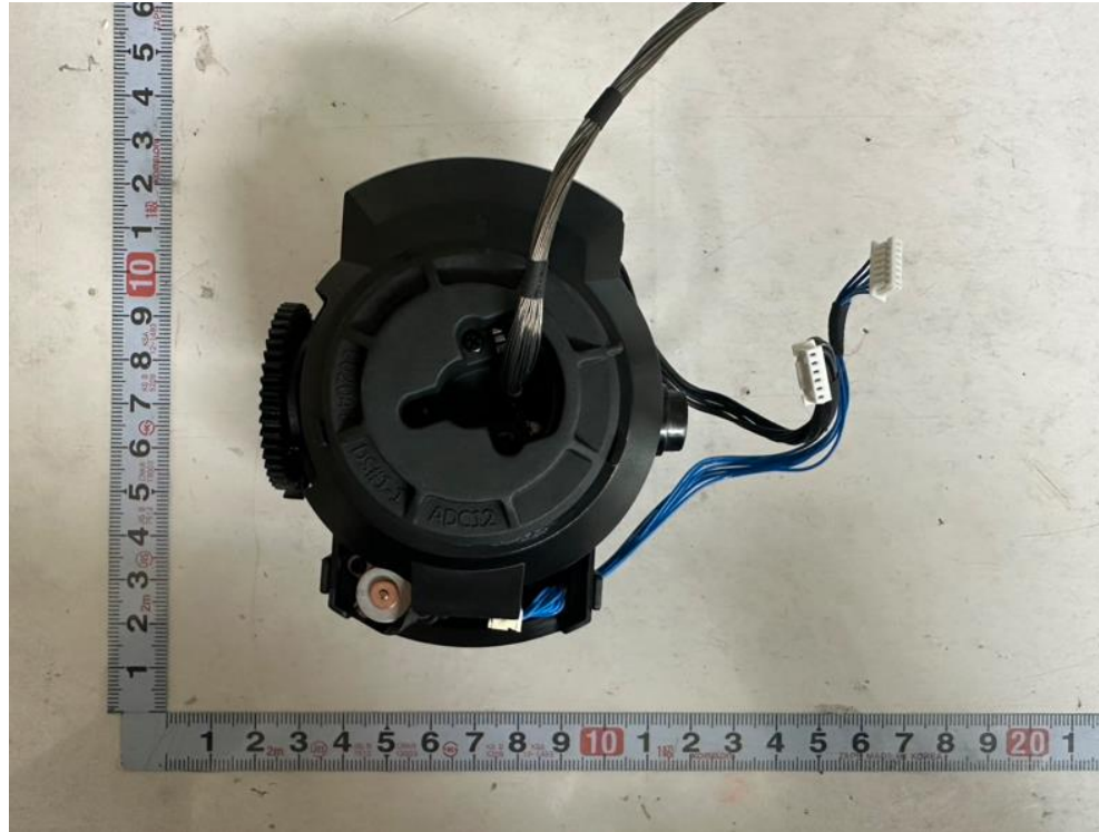
<Photo 8> Lens view 3
