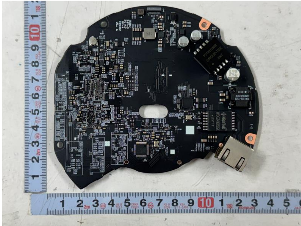
<Photo 10> Network board view 2
